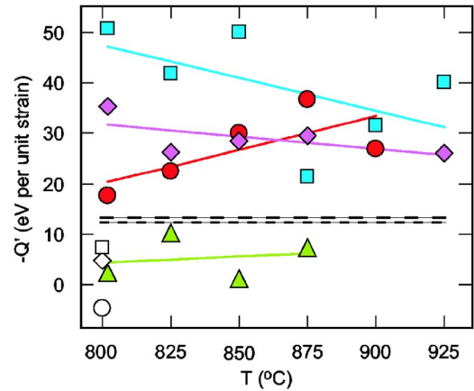
FIG. 6. (Color online) Biaxial strain coefficient vs T for various compositions determined by our analysis of the data of Zangenberg et al. (open symbols) and Kuo et al. (filled symbols) for boron diffusion in Si and Si-Ge alloys. Zangenberg data: open squares: 24% Ge, compressive; open diamonds: 12% Ge, compressive; open circles: 0% Ge, tensile; open triangles: 12% Ge, tensile. Kuo data: filled square: 20% Ge, compressive; filled diamond: 11% Ge (tensile and compressive); filled circle: 0% Ge, tensile. Sloping lines are linear fits to the data. Dashed lines are prediction of Eq. (39) with \tilde{A}=0 (Table II, sixth column) using our measured \tilde{V} values at 850 °C in Si (long dashed line) and \text{Si}_{89}\text{Ge}_{11} (short dashed line); dashed lines are drawn horizontal because there is insufficient information to predict a slope.
