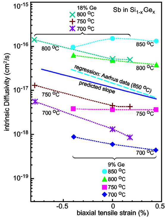
FIG. 5. (Color online) Strain effect on Sb diffusion in \text{Si}_{1-x}\text{Ge}_x at constant x and T ; data from Portavoce et al. Data series spanning strain range -0.4 – +0.45 % and identified by filled symbols are for x=0.09 ; series spanning range -0.8 – +0.2 % and identified by unfilled symbols are for x=0.18 . Dotted lines are to guide the eye. Long dashed line: regression of Aarhus data for x=0, 0.08 , and 0.10 to Eq. (44), used here to predict D for x=0.09, T=850 °C. Solid line: slope predicted for D^{\text{int}} at 850 °C from Eq. (39) assuming \tilde{A}=0 and \tilde{V} for alloys is the same as that measured for x=0 in this work; vertical offset is arbitrary.
