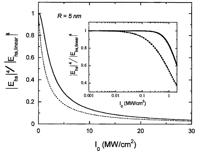
FIG. 10. Intensity dependence of SERS signal enhancement normalized to its linear (low intensity) value. The thick line represents the response of a single 5-nm particle at \lambda=420 nm, and the dotted line represents the peak value in the spatial distribution for a fractal consisting of 5 nm particles at \lambda=1260 nm. The insert shows the same on a semi-logarithmic scale.
