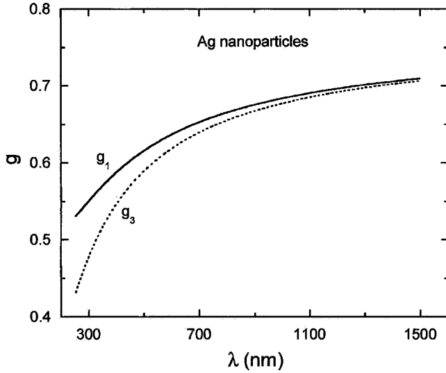
FIG. 1. Wavelength dependence of g_1 and g_3 for Ag particles.
