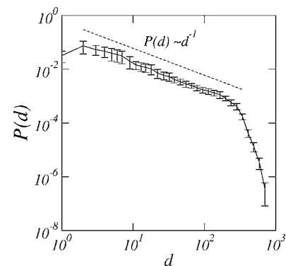
FIG. 8. Asymptotic distribution of the distance between spin deviations in a chain with N=800 spins. The regime for d < N/2 reflects the power-law decay of the wave-packet envelope. The fast decay for d > N/2 is related to the small probability of joint spin-deviation displacements. Error bars account for fluctuations over distinct disorder realizations.
