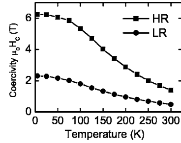
FIG. 9. Temperature dependence of the coercivity \mu_0 H_{c\perp} of as-annealed HR and LR Pr-Fe-B thin films.
