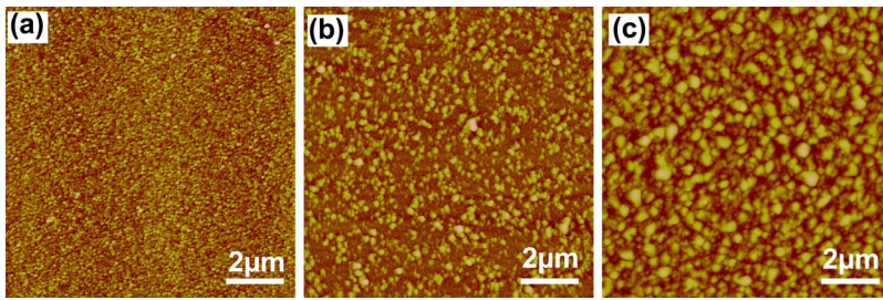
FIG. 3. (Color online) AFM images of as-sputtered Pr-Fe-B thin films with different deposition rates: (a) 0.5 nm/s, (b) 0.7 nm/s, and (c) 0.8 nm/s.
