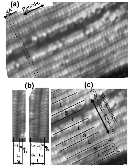
FIG. 2. (a) Collage of STM images ( 145 \times 90 \text{ Å} ) of two contiguous regions in the 2-fold Al-Ni-Co surface. The terraces are made of rows of periodically arranged atoms ( 4 \text{ Å} ) along the 10-fold direction and separated by distances L and S . (b) Expanded view showing the interior in the L and S sections. L contains two atomic rows, separated by L_2 and S_2 distances. S contains one row, at distances of L_2 and S_2 from the boundary. (c) The sequence of L and S spacings between rows follows a Fibonacci sequence. The trench in the center of (a) and (c) is due to a missing L+S section. The complete Fibonacci sequence of LSLSLLSLLS is visible in (a).
