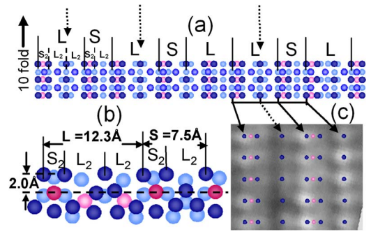
FIG. 4. (Color online) Atomic model of the 2-fold surface derived from the bulk x-ray diffraction model of Takakura et al. (Ref. 20). The Al is blue and transition metal (Ni, Co) is red. The plane shown here is the one containing only Al atoms, which provides the best fit with the experimental STM images. (a) Top view ( 8 \text{ Å} \times 90 \text{ Å} ). There three levels of color of the Al atoms corresponding to relative distances below the surface (dark=top; medium= -0.5 \text{ Å} , light= -2 \text{ Å} ). The spacing between Al atoms along the 10-fold direction is 4.1 \text{ Å} , and the sequence along the 2-fold direction shows the same Fibonacci sequence ( LSLSLLSL or S_2L_2L_2S_2L_2S_2L_2L_2S_2L_2L_2S_2L_2L_2S_2L_2L_2S_2L_2L_2 ) as the STM image in Fig. 2(c). Dashed arrows mark the positions of local mirror planes. (b) A cross section showing the atomic arrangement perpendicular to the surface (perpendicular to the 10-fold direction). A transition metal rich layer is visible below ( \sim 2.0 \text{ Å} lower) the topmost Al one. (c) A STM image of section of L and S with the Al sites indicated by blue dots.
