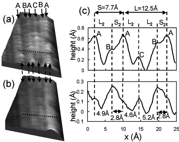
FIG. 3. STM images of the same area acquired at positive and negative bias. (a) V_s = +1.2 V, I = 0.1 nA (b) V_s = -1.2 V, I = 0.1 nA. (c) Line profiles across the dashed lines in (a) and (b) reveal three electronically different atomic rows, labeled A, B, and C.
