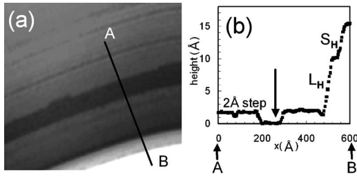
FIG. 1. (a) 650 \times 650 \text{ Å} STM image of the 2-fold Al-Ni-Co surface ( V_s = 1.0 \text{ V} , I_t = 0.1 \text{ nA} ). Steps and terraces composed of rows of atoms are visible. (b) Line profile showing steps with heights 4.7 \text{ Å} ( S_H ), 7.8 \text{ Å} ( L_H ), and 1.9 \text{ Å} . The ratio of L_H to S_H is approximately equal to the golden mean (1.618), characteristic of aperiodic quasicrystalline structure. The lowest terrace, indicated by the arrow in (b), is a domain where the periodicity along the rows is 8 \text{ Å} . In the other terraces the periodicity along the rows is 4 \text{ Å} .
