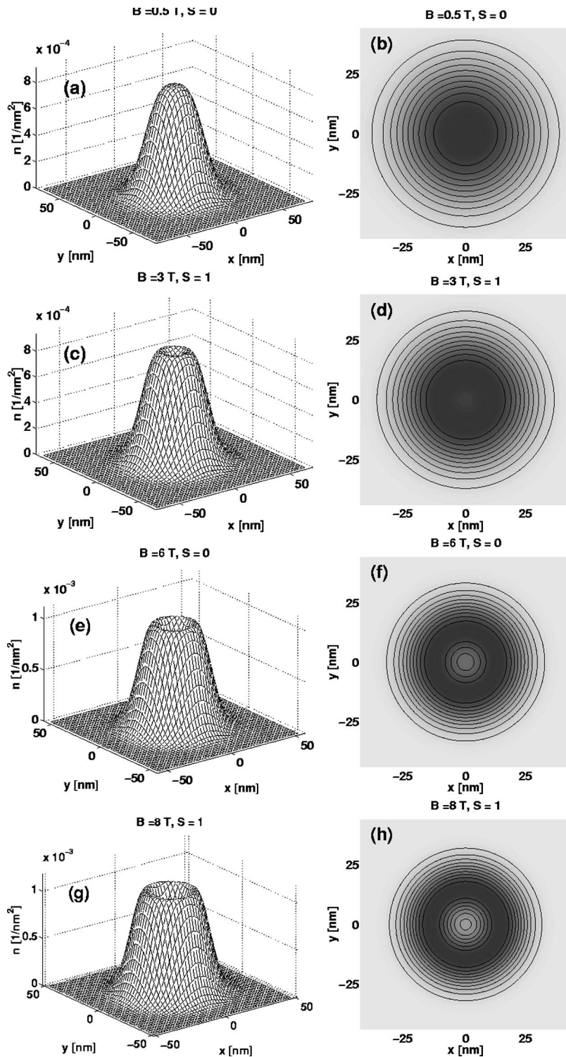
FIG. 7. Total electron density of the ground state at different magnetic field values for the parabolic ( L_x=L_y=0 ) QD. In the left column are densities in 1/\text{nm}^2 and on the right column are contours of the densities. Dark regions in the contours mark high density and brighter regions low density. Notice that in the densities the scale in the x and y axes is changing and the height of the peak is increasing with magnetic field. The range of axes in the contour plots is kept fixed. The magnetic field value and the spin type of the ground state are plotted above each subfigure.
