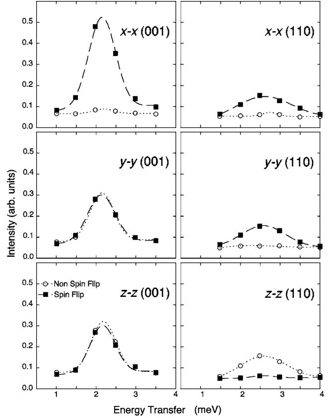
FIG. 3. Constant- \mathbf{Q} scans taken at (001) (left-hand side) and (110) (right-hand side). The neutron x - x , y - y , and z - z spin-flip (SF, black squares) and non-spin-flip (NSF, open circles) cross sections are shown. The error bars are smaller than the point size.
