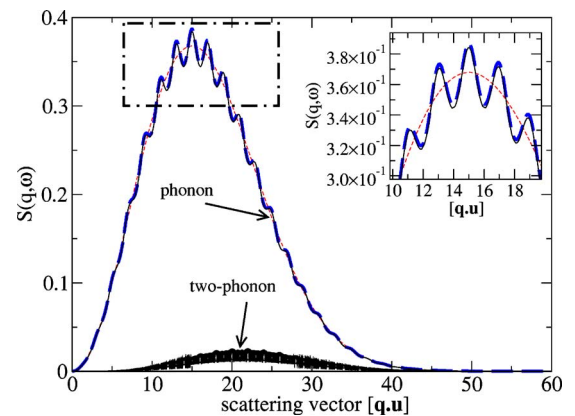
FIG. 4. (Color online) A plot of the coherent inelastic S(q, \omega) profile versus q = [\mathbf{q} \cdot \mathbf{u}] , for phonon in a harmonic lattice: C=0.05 , A_3=A_4=0 . The thin dashed line has been obtained by a perturbation theory. The thin solid line corresponds to our numerical treatment and the thick dashed line to a plot of the exact formula (see Ref. 4) (the two latest curves are hardly distinguished in the graph). In the inset, the area in the dot-dashed rectangle is magnified. The X axis unit is \pi/a_0 .
