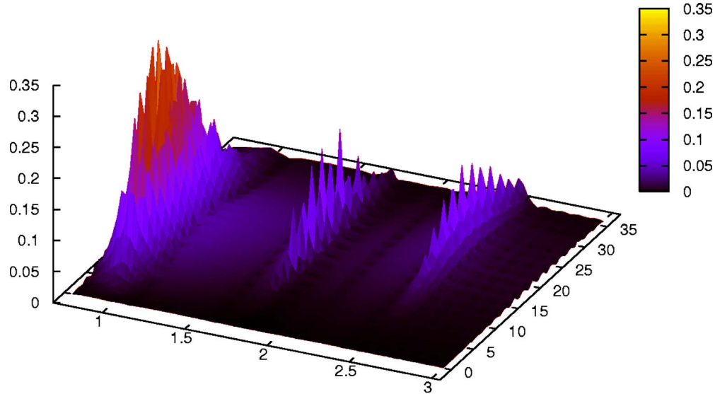
FIG. 2. (Color online) A 3D plot of the inelastic S(q, \omega) as a function of the dimensionless energy transfer \omega and the scalar product q = [\mathbf{q} \cdot \mathbf{u}] of the transfer momentum \mathbf{q} and the polarization \mathbf{u} . The parameters are the same as in Figs. 1(a) and 1(b). The figure is easier to depict in color.
