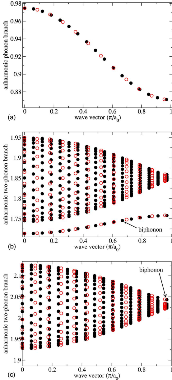
FIG. 1. (Color online) energy spectrum of a chain composed of N unit cells, N=33 (full circles) and N=23 (empty circles): (a) the optical phonon branch for model parameters C=0.05 , A_3=0.12 and A_4=0.01 ; (b) the two-phonon energy region for the same parameters as (a); (c) the same as in (b) but for C=0.05 , A_3=0.05 and A_4=0.01 . The Y axis unit is \hbar\Omega . The wave vector is reported on the X axis, whose unit is (\pi/a_0) and ranges over the lattice first Brillouin zone.
