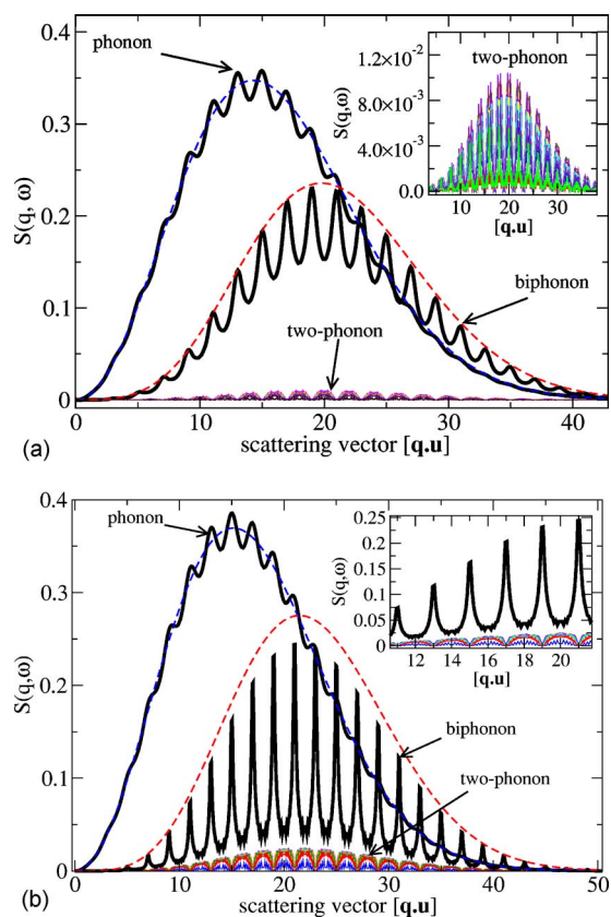
FIG. 5. (Color online) A plot of the coherent inelastic S(q, \omega) profile versus q=[\mathbf{q}\cdot\mathbf{u}] , for phonon, biphonon, and two-phonon states. The model parameters are: (a) C=0.05 , A_3=0.12 , and A_4=0.01 ; (b) C=0.05 , A_3=0.05 , and A_4=0.01 . The dashed lines correspond to our perturbation theory and the solid lines to our numerical treatment. The X axis unit is \pi/a_0 and the scattering vector q ranges over 60 Brillouin zones. The inset shows a magnification of the two-phonon contributions.
