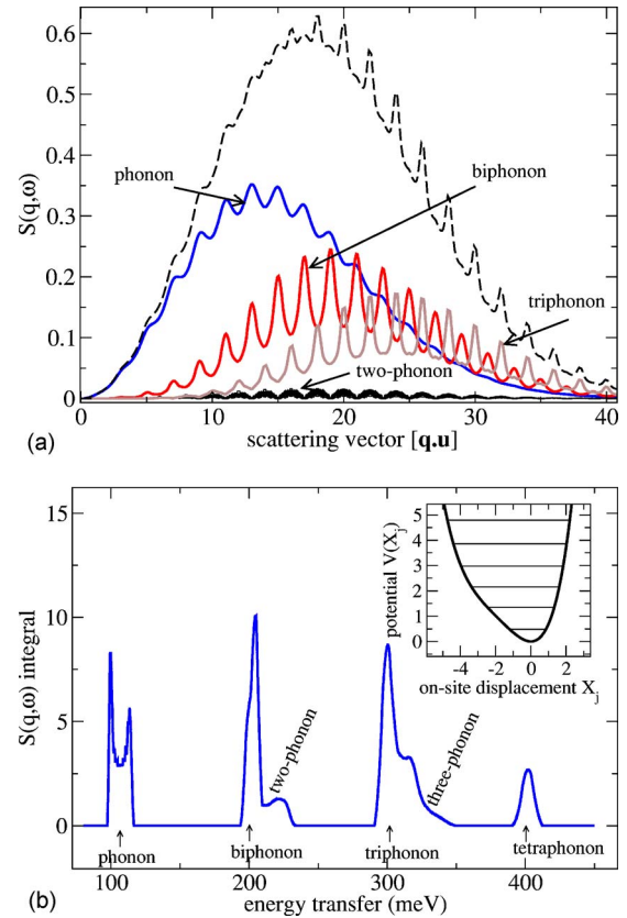
FIG. 6. (Color online) In (a), the same as in Fig. 5(a) but for different model parameters: C=0.06 , A_3=0.17 , and A_4=0.0231 . In addition, have been plotted the S(q, \omega) profile for the triphonon and the integral of S(q, \omega) over the energy transfer \omega (dashed line). The elastic contribution has been skipped. In (b), a plot of the profile of the S(q, \omega) integral over the reciprocal lattice (see text), vs the energy transfer \omega , for same parameters as in (a). The inset in (b) shows the corresponding potential landscape V(X_j) and its quantum levels. Our energy unit \hbar\Omega has been fixed to 107 meV.
