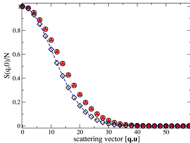
FIG. 3. (Color online) A plot of the Debye-Waller factor [S(q, \omega=0)/N] vs the scalar product q = [\mathbf{q} \cdot \mathbf{u}] , for different model parameters. Each symbol corresponds to a Bragg peak. Our numerical results are reported for C=0.05 , A_3=A_4=0 (diamonds), and C=0.05 , A_3=0 , A_4=0.2 (triangles). The exact formula derived in a harmonic model (dashed line) confirms the former while the latter has been computed within a perturbation theory (circles) too. The X axis, which unit is \pi/a_0 bears the scattering vector q over a range of 60 Brillouin zones.
