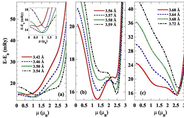
FIG. 2. (Color online) Magnetic moment dependence of the total energy E-E_0 for \gamma -Fe at several selected lattice parameters, showing the three distinct regimes. The inset in (a) shows the calculated values of E-E_0 around the minimum LS state.
