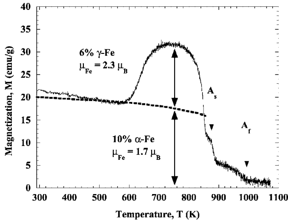
FIG. 1. Temperature dependence of the measured magnetization for \text{Fe}_{16}\text{Cu}_{84} . The dashed line corresponds to the contribution associated with \alpha -Fe (Ref. 15). A_s and A_f represent the starting and final temperatures of the martensite-austenite transformation.
