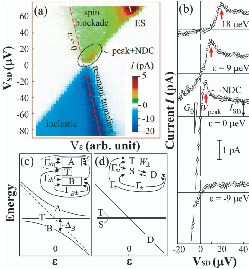
FIG. 3. (Color) (a) Current I as a function of V_\varepsilon and V_{SD} at \delta=0 . Note that the color scale is different for positive and negative current. (b) I - V_{SD} curves at some constant \varepsilon , extracted from (a). The arrows indicate the peak position V_{\text{peak}} (unit: \mu\text{V} ). (c) The anticrossing energy diagram for the two-electron DQD with coherent interdot coupling. The inset shows the cotunneling transitions between the energy levels. (d) Schematic energy diagram of the DQD with incoherent interdot coupling. The inset shows some possible transitions between the two-electron charge states.
