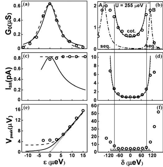
FIG. 4. Zero-bias conductance G_0 (a) and (b), spin blockade current I_{SB} (c) and (d) at V_{SD} = 50 \mu\text{V} and current peak position V_{\text{peak}} (e) and (f) as a function of \varepsilon and \delta . Note that (a), (c), and (e) are obtained at \delta=0 and that (b), (d), and (f) are for \varepsilon=0 . The solid and dashed curves were calculated considering coherent and incoherent interdot coupling, respectively. The dash-dotted Lorentzian curves in (b) are guides for the sequential tunneling regions and the electrostatic coupling energy U = 255 \mu\text{eV} is determined from the energy spacing between peaks A and B. The dotted line in (e) is a reference for eV_{\text{peak}} = \varepsilon . The cotunneling region is confined to the \delta range of -90 to 90 \mu\text{eV} (between the two solid straight lines).
