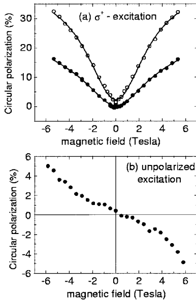
FIG. 2. (a) Dependence of the degree of circular polarization of the PL emission on a magnetic field under circularly polarized excitation. Open circles correspond to data detected at \lambda=5455 \text{ \AA} ; full circles to detection at \lambda=5600 \text{ \AA} . (b) The same as (a) but observed with unpolarized excitation, with detection at \lambda=5600 \text{ \AA} .
