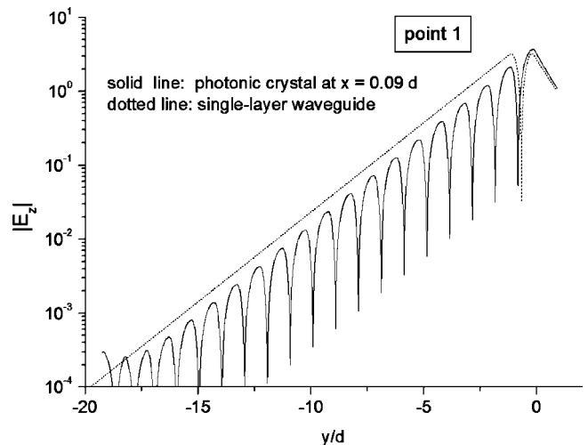
FIG. 12. Comparison between the fields in the photonic crystal structure and in the simple model that consists in one homogeneous guiding layer. TE polarization.
