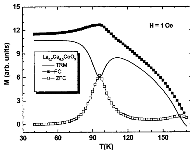
FIG. 2. Temperature dependence of TRM, FC, and ZFC magnetization, M , recorded for \text{La}_{0.7}\text{Ca}_{0.3}\text{CoO}_3 at H=1 Oe.
