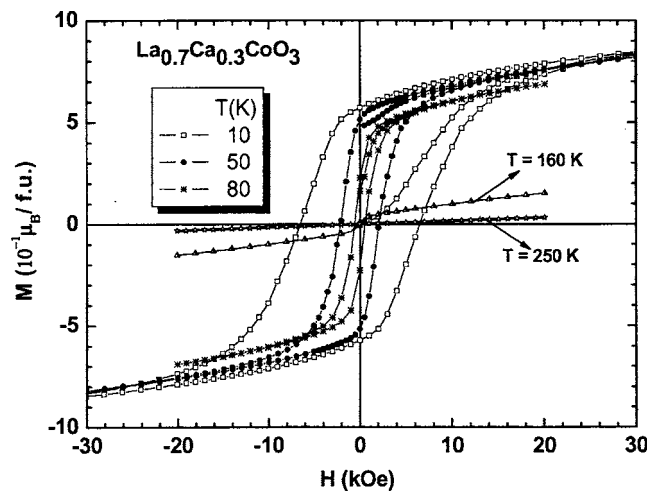
FIG. 4. Typical hysteresis curves for \text{La}_{0.7}\text{Ca}_{0.3}\text{CoO}_3 at different temperatures.
