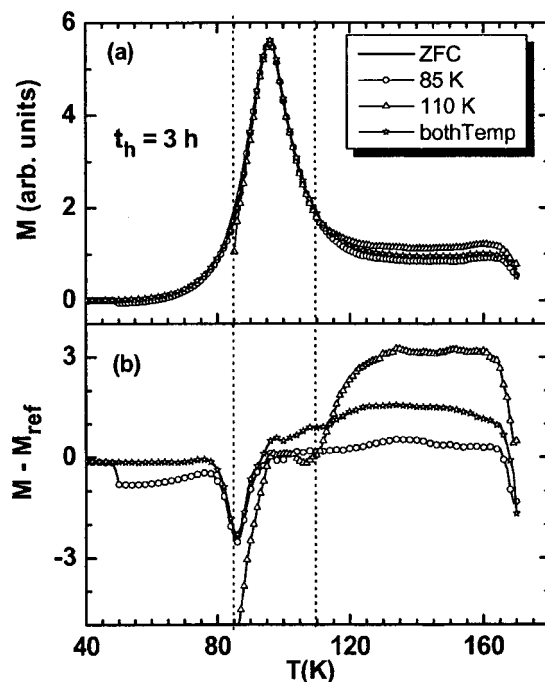
FIG. 10. ZFC magnetization memory experiment on \text{La}_{0.7}\text{Ca}_{0.3}\text{CoO}_3 ; (a) the temperature dependence of ZFC magnetization, M (reference curve), and on imprinting memories of two temperature stops (at 85 and 110 K) during cooling each for 3 h and (b) the difference ( M - M_{ref} ) plot of the respective curves.
