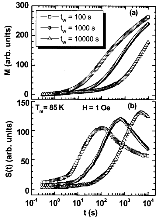
FIG. 8. ZFC relaxation measurements on \text{La}_{0.7}\text{Ca}_{0.3}\text{CoO}_3 at T_m = 85 K for different waiting times, t_w = 100, 1000, and 10000 s ( H = 1 Oe).
