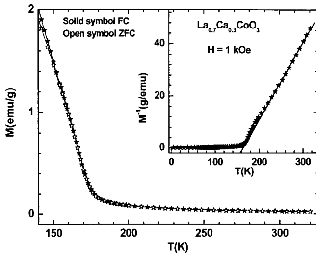
FIG. 3. Temperature dependence of the ZFC and FC magnetization, M , of \text{La}_{0.7}\text{Ca}_{0.3}\text{CoO}_3 ( H=1000 Oe). The inset shows the temperature dependence of inverse magnetization, M^{-1} , ( H=1000 Oe).
