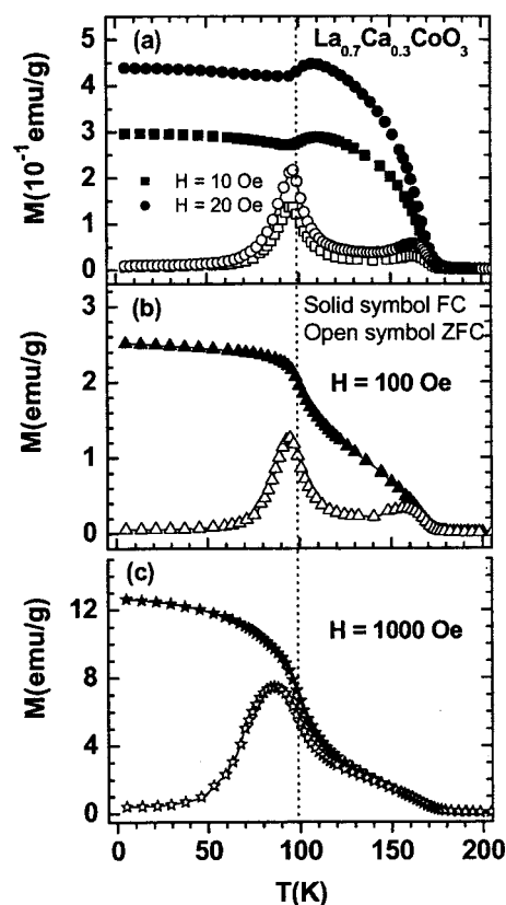
FIG. 1. Temperature dependence of the ZFC and FC magnetization, M , of \text{La}_{0.7}\text{Ca}_{0.3}\text{CoO}_3 at different applied fields. (a) H=10, 20 Oe; (b) H=100 Oe; and (c) H=1000 Oe. ZFC data in open symbol and FC data in solid symbol.
