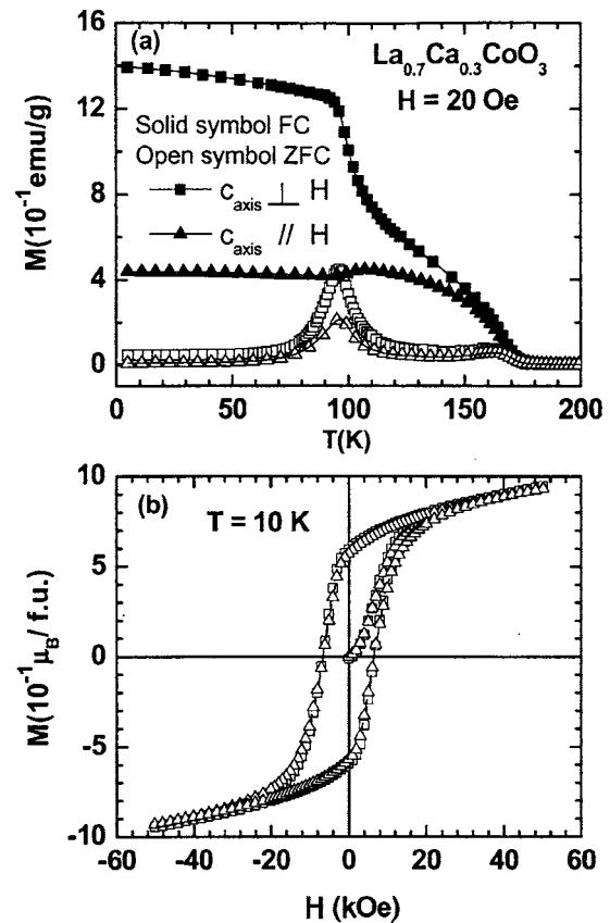
FIG. 5. Variation of (a) the ZFC and FC magnetization, M ( H=20 Oe); and (b) magnetic hysteresis curves of \text{La}_{0.7}\text{Ca}_{0.3}\text{CoO}_3 for different field directions.
