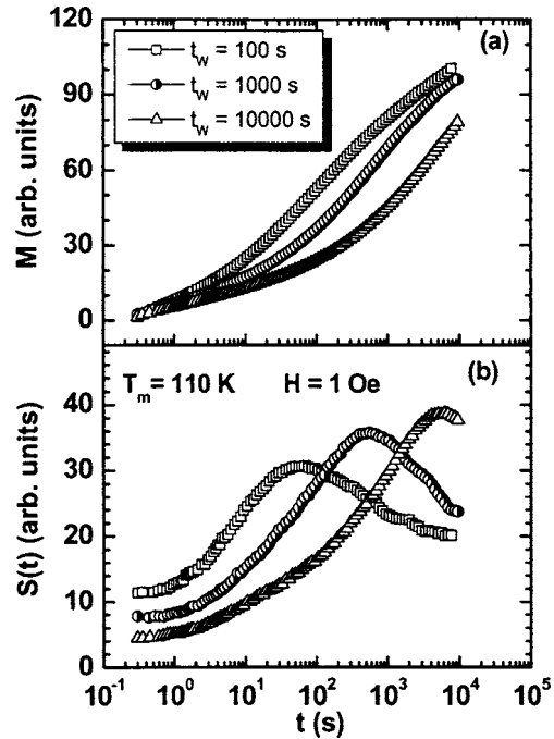
FIG. 9. ZFC relaxation measurements on \text{La}_{0.7}\text{Ca}_{0.3}\text{CoO}_3 at T_m = 110 K for different waiting times, t_w = 100, 1000, and 10000 s ( H = 1 Oe).
