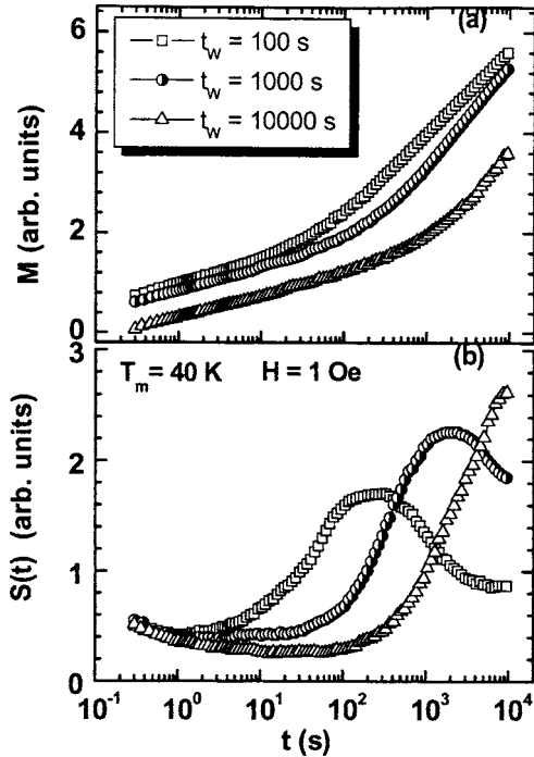
FIG. 7. ZFC relaxation measurements on \text{La}_{0.7}\text{Ca}_{0.3}\text{CoO}_3 at T_m = 40 K for different waiting times, t_w = 100, 1000, and 10000 s ( H = 1 Oe).
