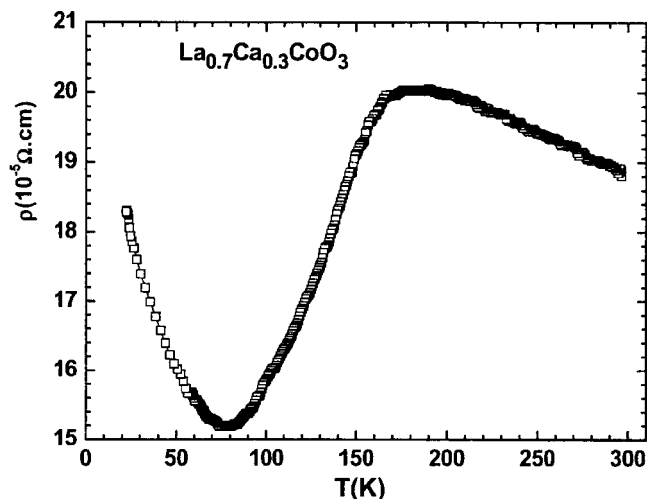
FIG. 11. Temperature dependence of electrical resistivity, \rho , of \text{La}_{0.7}\text{Ca}_{0.3}\text{CoO}_3 .
