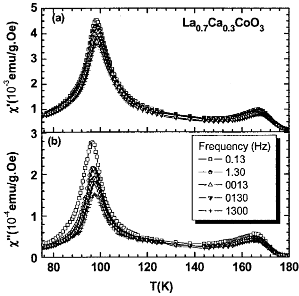
FIG. 6. The temperature dependence of the (a) in-phase and (b) out-of-phase ac susceptibility of \text{La}_{0.7}\text{Ca}_{0.3}\text{CoO}_3 at different frequencies.
