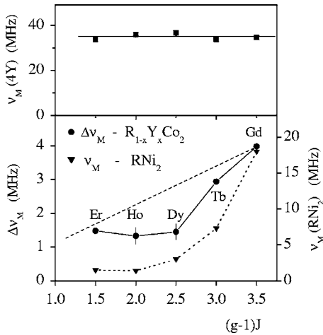
FIG. 6. Parameters \nu_M(4Y) (top section) and \Delta\nu_M (bottom section) describing the dependence of the magnetic frequencies \nu_M^j of ^{111}\text{Cd}:R_{1-x}Y_x\text{Co}_2 on the number n_R of nearest R neighbors of the probe nucleus versus the spin projection (g-1)J . \nu_M(4Y) and \Delta\nu_M were determined by fitting Eq. (4) to the data in Fig. 5. The dashed line illustrates a linear spin dependence of \Delta\nu_M . In addition, the bottom section also shows the spin dependence of the magnetic hyperfine frequency of ^{111}\text{Cd} in \text{RNi}_2 (right-hand scale).
