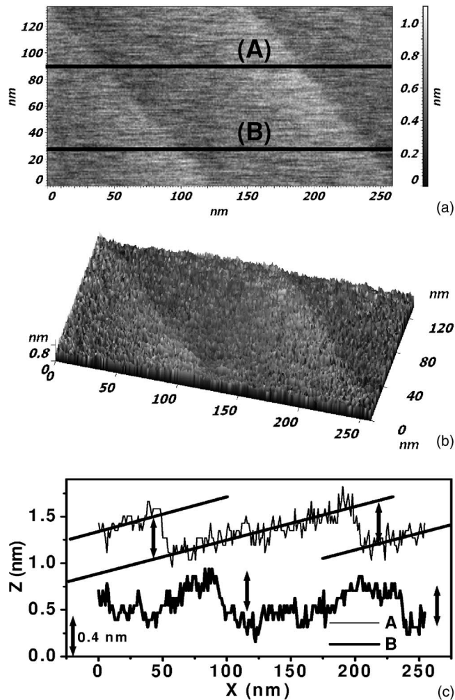
FIG. 3. (a) Topographic two-dimensional (2D) and (b) three-dimensional (3D) images of a selected region containing two monolayer steps/edges (staircaselike) on the surface of the HOPG sample. (c) Two height profiles along the lines marked in (a) as A and B. The arrows indicate the 0.4 nm step height. [Note: The tilt in the step (line profile) is an artifact of processing (linear line fit along the scan x direction).]
