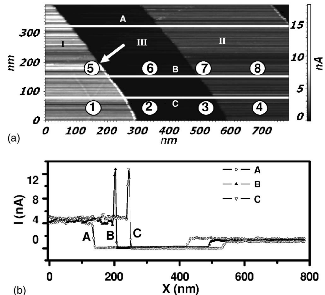
FIG. 6. (a) Local conductance map for the forward bias condition. Labels 1 to 8 are the spots where current vs voltage ( I-V ) measurements were carried out. (b) The current profile along the lines marked in (a) with labels A to C for forward bias condition. The arrow indicates the bright streak abruptly ending along the edge for the forward bias condition on the same ribbon.
