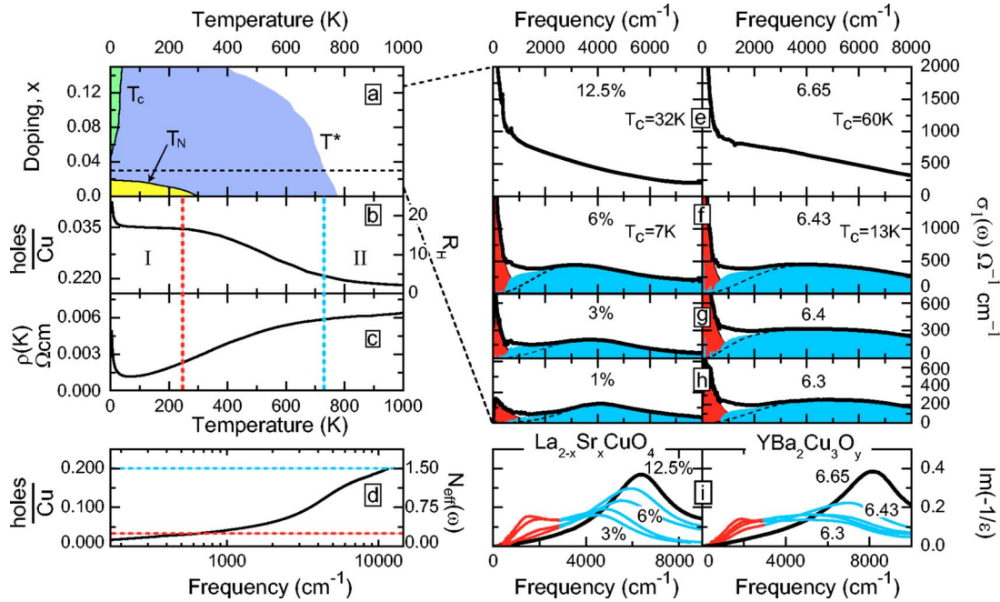
FIG. 1. (Color online) Optical data for YBCO and both optical and transport data for LSCO discussed in the context of the high- T_c phase diagram. Left panels are data for x=0.03 LSCO and right panels depict the low temperature optical conductivity as a function of doping for both LSCO and YBCO. Data in panels (f)–(h) are at T=7 K and at T just above T_c in panels (e). Panel (a): phase diagram with the values shown for LSCO; the yellow area is the long range AF region (denoted by T_N ), the green area is the superconducting region (marked by T_c ), and the pseudogap region is denoted by T^* . To facilitate a direct comparison with the data, temperature is plotted on the horizontal axis and doping on the vertical axis. The Hall coefficient R_H ( 10^{-3} \text{cm}^3/\text{C} ) displayed in panel (b) reveals two characteristic regimes (I and II). This is exemplified for the x=0.03 sample but similar behavior is found for all heavily underdoped crystals. These regimes can also be identified with significant regions in the dc resistivity corrected for thermal expansion (c). Panel (d): the effective number of carriers, N_{\text{eff}} ( 10^6 \Omega^{-1}\text{cm}^{-2} ), determined from the optical data as described in the text. Right panels: the real part of the conductivity at low temperature [ T=10 K, except T=T_c for (e) and (f) and T=150 K for y=6.65 ], displayed as black solid curves. Red colors signify fits using the standard Drude model. The blue area is a subtraction of the Drude fit from \sigma_1(\omega) and is referred to as the “mid-infrared contribution” throughout the text. The resonant structure in the latter contribution can be adequately described with a Lorentzian oscillator (dashed lines). The loss function [\text{Im}(-1/\epsilon)] , panels (i), also clearly depicts two components (shown as red and blue curves) for dopings x < 0.10, y < 6.65 , and the progression to a single component, (black solid curve) for higher dopings.
