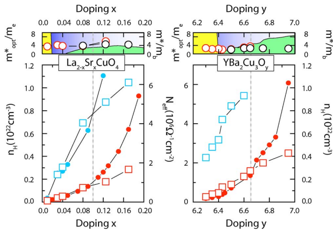
FIG. 2. (Color online) Top panels show the optical effective mass as determined by the methods described in the text. Red symbols are the mass determined using a combination of optics and transport (left axis labels), and the black symbols represent the mass determined within the extended Drude model (right labels). All methods produce consistent results and mass values which are doping independent over large regions of the phase diagram. The low temperature long-range AF ordered phase is denoted by the yellow shaded area and SC region by the green area. Note that despite the formation of the AF regime near the Mott transition, there is no noticeable enhancement of the optical mass. Bottom panels show both the effective spectral weight from optics data (red and blue open squares) and the number of holes as determined by transport (red and blue dots).
