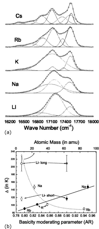
FIG. 2. (a) Absorption spectra for hypersensitive transition in 30\text{R}_2\text{O}-69.5\text{B}_2\text{O}_3-0.5\text{Nd}_2\text{O}_3 glasses ( \text{R}=\text{Li}, \text{Na}, \text{K}, \text{Rb}, \text{Cs} ). (b) Variation of \Delta with alkali mass number (top x -axis, and \circ ) and with basicity moderating parameter (AR) (bottom x -axis, and \bullet ). The dotted line is a guide to the eye and the solid line is a linear fit to the \Delta values.
