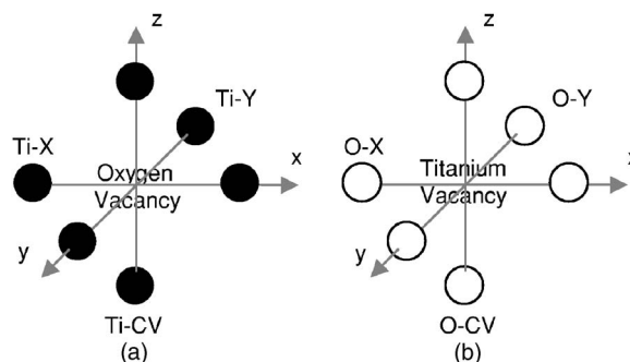
FIG. 2. Schematic representation of (a) O vacancy and (b) Ti vacancy.
