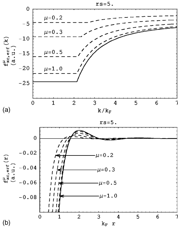
FIG. 13. The static exchange-correlation kernel f_{xc,erf}^{\mu} in reciprocal [Eq. (25)] and direct [Eq. (26)] spaces for r_s=5 with the erf interaction (dashed curves) for \mu=0.2, 0.3, 0.5, and 1.0 . For comparison, the case of the Coulomb interaction (solid curve) is also shown.
