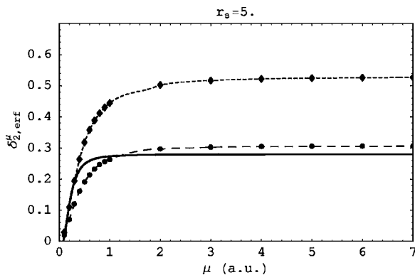
FIG. 9. \delta_{2,\text{erf}}^\mu with the erf interaction for r_s=5 : formula from virial theorem [thick solid curve, Eq. (A6)], RPA (short-dashed curve), and G_0W_0 (long-dashed curve) calculations.
