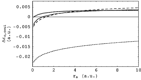
FIG. 14. The error in the correlation energy \Delta\varepsilon_{c,coul} = \varepsilon_{c,coul}^{ACFD} - \varepsilon_{c,coul} for the Coulomb interaction [Eq. (27)] with different exchange-correlation kernels: RPA ( f_{xc}=0 , short-dashed curve), MCS (Ref. 30) (solid curve), and CDOP (Ref. 31) (dotted curve) parametrizations and the simple interpolation formula [Eq. (25), long-dashed curve].
