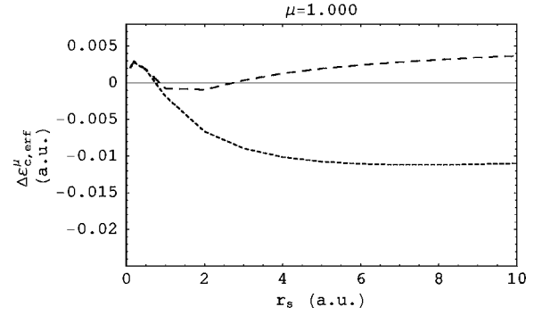
FIG. 15. The error in the correlation energy \Delta\varepsilon_{c,erf}^{\mu} = \varepsilon_{c,erf}^{\mu,ACFD} - \varepsilon_{c,erf}^{\mu} for the erf interaction [Eq. (29)] with different exchange-correlation kernels: RPA ( f_{xc}=0 , short-dashed curve), the simple interpolation formula [Eq. (25), long-dashed curve], for \mu=1 .
