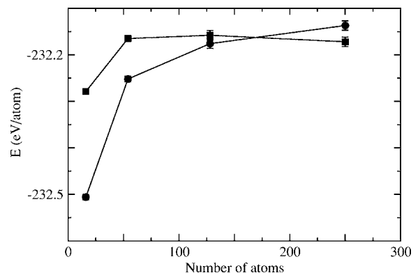
FIG. 2. The DMC energy per atom for MgO in the rocksalt structure with a volume per atom of 9.06 Å 3 as a function of the number of atoms in the repeating cell, using both the Ewald interaction (circle) and the MPC interaction (squares).
