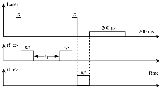
FIG. 4. Timing of the laser beam and the radio frequency fields. The top trace shows the laser pulses, the center trace the radio frequency pulses that are resonant with the excited state m = \pm\frac{1}{2} \leftrightarrow \pm\frac{3}{2} transition, and the bottom trace the pulses that are resonant with the corresponding ground state transitions. The detection uses a weak laser pulse for Raman heterodyne detection of the ground state nuclear spin coherence.
