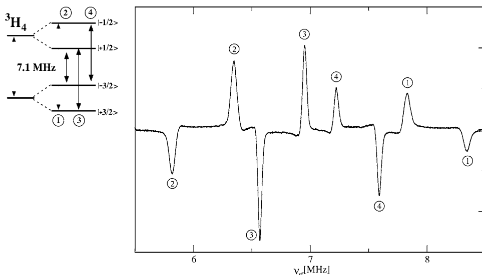
FIG. 2. Raman heterodyne spectrum for the ^3H_4 |\pm \frac{1}{2}\rangle \leftrightarrow |\pm \frac{3}{2}\rangle transition of \text{Pr}^{3+}:\text{YAlO}_3 at 3 K. The external magnetic field for this configuration is listed in Table II. Two inequivalent sites lead to eight transitions in the spectrum.
