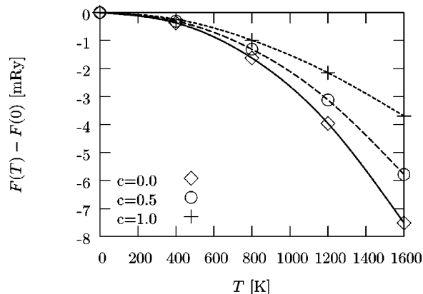
FIG. 16. Temperature dependence of the electronic free energy, as defined in the text.
