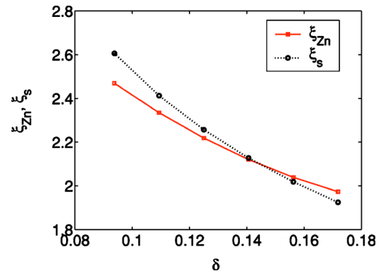
FIG. 4. (Color online) The size of the spatial distribution of the local moments, \xi_{Zn} (solid), and the bulk spin correlation length, \xi_s = \sqrt{2}/\delta\pi (dotted), vs doping \delta .
