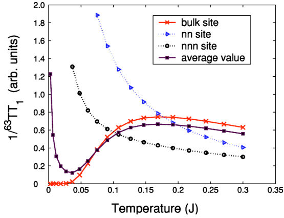
FIG. 5. (Color online) Contributions to 1/^{63}T_1T from different sites are calculated. Solid curve with crosses: from the site far from the zinc impurity. Dashed curve with triangles: the nn site near the zinc. Dashed curve with circles: the next-nearest-neighbor (nnn) site near the zinc. Solid curve with squares: average over all sites in a 16 \times 16 lattice with one zinc (see text).
