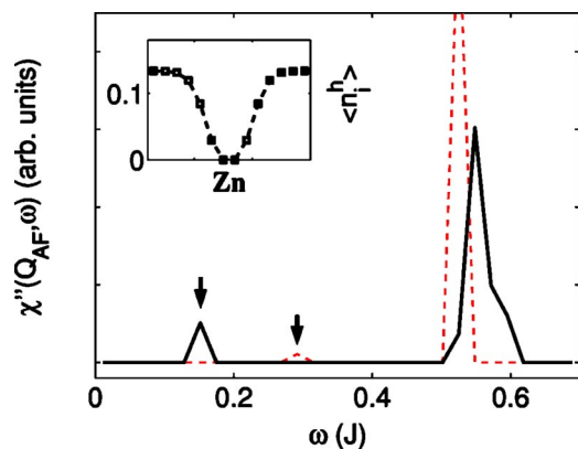
FIG. 9. (Color online) Dynamic spin susceptibility at Q_{AF} = (\pi, \pi) is shown as the solid curve when the holon density is suppressed locally around the zinc (see the inset). For comparison, the dashed curve illustrates the case for a uniform holon density distribution.
