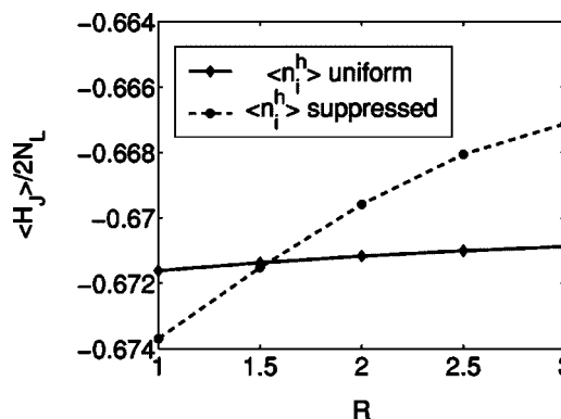
FIG. 11. The average superexchange energy \langle H_J \rangle / (2N_L) per bond ( N_L denotes the total number of lattice sites excluding the zinc sites) as a function of the parameter R in (24). Solid curve: uniform holon distribution. Dashed curve: locally suppressed holon density around the zinc indicated by the inset of Fig. 10.
