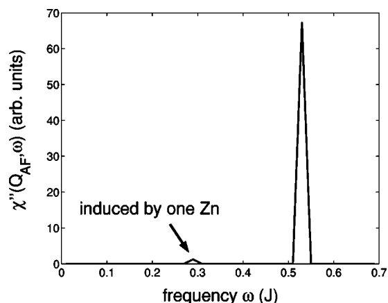
FIG. 8. Dynamic spin susceptibility at AF wave vector Q_{AF} = (\pi, \pi) with \delta=0.125 . The high-energy resonancelike peak at E_g \approx 0.53J is from the bulk (zinc free) state, while the low-energy excitations indicated by the arrow are the ones induced by the zinc impurity.
