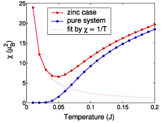
FIG. 7. (Color online) Uniform spin susceptibility in the pure system is shown by the solid curve with full circles. The case with one zinc is illustrated by the solid curve with triangles. The dashed curve is a fit by \chi = 0.2390/T .
