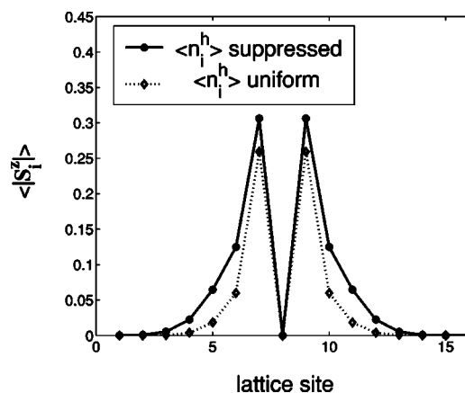
FIG. 10. The distribution of \langle S_i^z \rangle , corresponding to the profile of the holon density shown in the inset of Fig. 9, is plotted as the solid curve, as compared to the dashed curve for the uniform holon distribution.
