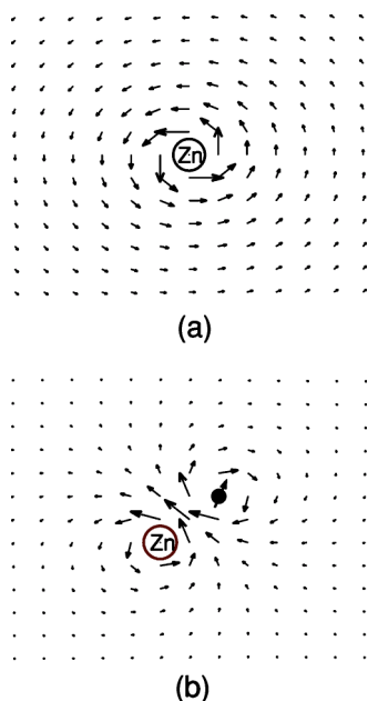
FIG. 1. (a) A vacancy (zinc impurity) always induces a vortexlike supercurrent response in the superconducting phase due to the phase string effect. (b) To compensate such a vortex effect, a spinon, which carries an antivortex, has to be trapped around the zinc impurity, giving rise to a local S=1/2 moment.
