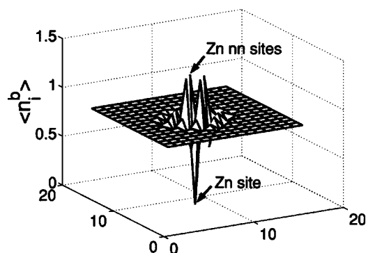
FIG. 2. Spinon density distribution \langle n_i^b \rangle = \langle \sum_\sigma b_{i\sigma}^\dagger b_{i\sigma} \rangle around the zinc impurity. The lattice is 16 \times 16 with doping \delta=0.125 .
