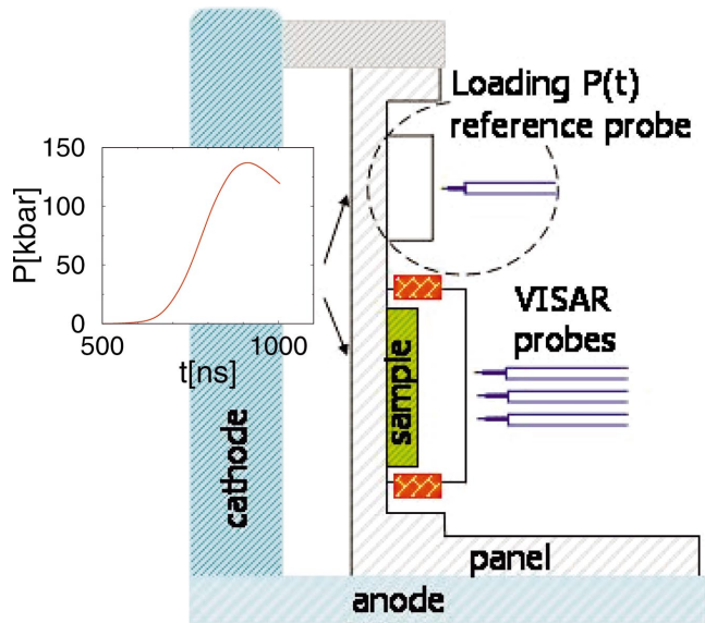
FIG. 1. Schematic cross section through target assembly. The Bi sample is contained between the panel (Cu or Al) and the transparent window (LiF or Sapphire). Heat is applied to the sample through a band heater (red) wrapped around the circumference of the window. A 3-mm vacuum gap (AK gap) exists between the panel and cathode. A rapidly varying magnetic field in the AK gap generates the pressure pulse that compresses the Bi sample. A reference probe assembly consisting of a transparent window impedance matched and glued to the panel provides a direct measurement of the loading pressure profile for each sample [see inset P(t) ].
