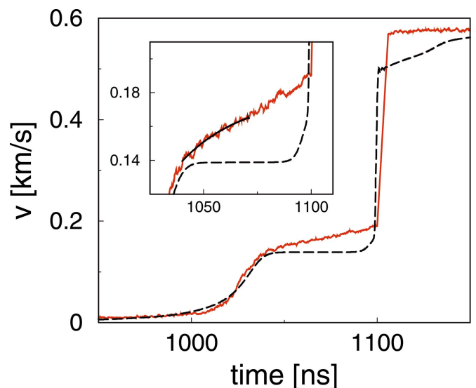
FIG. 3. VISAR trace (interface velocity) for a LiF window experiment: red line; hydrodynamic simulations: dashed black line. Inset: a blow-up of the reduced acceleration regime and kinetics fit (see text): solid black line.
