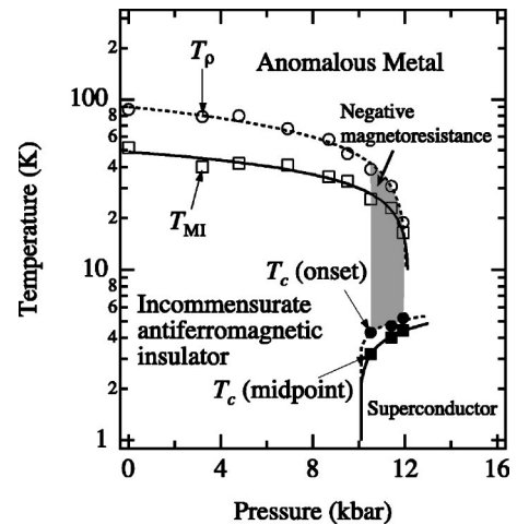
FIG. 5. The phase diagram of (MDT-TS)(AuI 2 ) 0.441 . The solid and dotted lines are guides to the eye.
