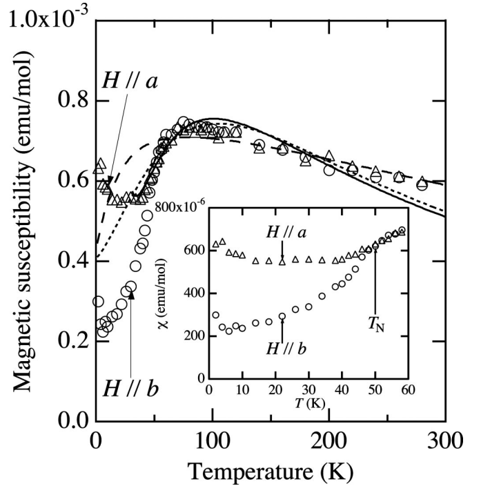
FIG. 4. Temperature dependence of the static magnetic susceptibilities ( H \parallel a and H \parallel b ). The dotted line is the 1D Heisenberg model ( J = -85 K and \mu_{\text{eff}} = 0.76 \mu_B ), the solid line is the 2D square lattice model ( J = -110 K and \mu_{\text{eff}} = 0.77 \mu_B ), and the dashed line is the 2D triangular lattice model ( J = -209 K and \mu_{\text{eff}} = 1.1 \mu_B ) fitted to the observed data of H \parallel b , under g = 2.0 . The inset shows the data in the low-temperature region.
