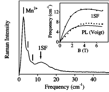
FIG. 6. Raman spectrum in the Voigt configuration for B=2.6 T and T=3.5 K. The laser energy is 1.66 eV. Bars indicate the manganese PR and its overtones. The peak labeled 1SF at \sim 12 \text{cm}^{-1} is the spin-flip transition of electrons bound to donors. The magnetic field dependence of the 1SF frequency is shown in the inset together with the PL shift in the Voigt configuration. Curves are theoretical predictions, Eq. (15), with x=0.004 .
