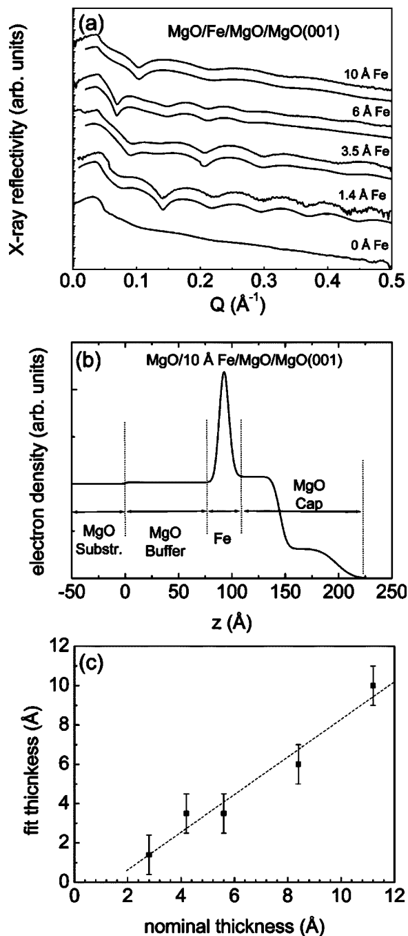
FIG. 2. (a) X-ray reflectivity data and best fit for a series of MgO/Fe/MgO samples with variable Fe thickness (the best fit is shown below the corresponding experimental curve). The indicated Fe thicknesses are those extracted from fits. The reflectivity for a sample with MgO buffer and capping layers deposited under equivalent conditions but with no Fe deposition (labeled as 0 Å Fe) is also shown as a reference. (b) The electron density profile obtained from the fit of a representative sample. MgO electron density is 6.67 \times 10^{23} electrons/cm 3 . (c) Fe thickness extracted from fits to XRR data versus the nominal Fe thickness.
