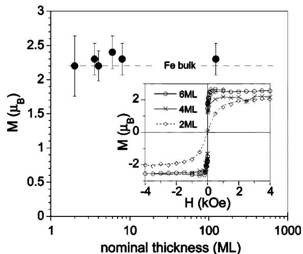
FIG. 4. The calculated magnetic moment as a function of the film thickness. Inset: in-plane hysteresis loops for the 2 ML, 4 ML and 6 ML samples from SQUID measurements at RT, once the background from the MgO substrate and capping layers has been subtracted. The dashed line for the 2 ML curve is the fit to the Langevin equation.
