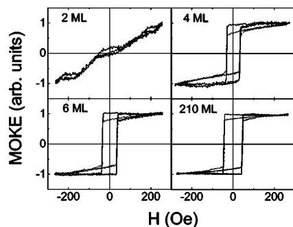
FIG. 3. In-situ transverse Kerr hysteresis loops with the magnetic field applied along different directions (easy [100] Fe axis, hard [110] Fe axis) for 2 ML, 4 ML, 6 ML and 210 ML samples.
