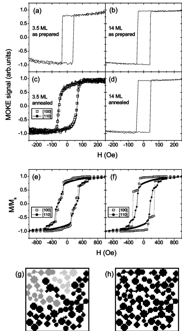
FIG. 8. (a)–(d) In-situ transverse Kerr hysteresis loops for different Fe thin films. (a) 3.5 ML sample, as prepared. The field is applied along the [100] direction; (b) 14 ML sample, as prepared. The field is applied along the [100] direction; (c) 3.5 ML sample after annealing at 400 °C. The two curves have been obtained with the field applied along the [100] and [110] directions; (d) 14 ML sample after annealing at 400 °C. The field is applied along the [100] direction. (e)–(f): simulated hysteresis loops for an ensemble of seventy-six iron particles. (e) The particles are interconnected forming three clusters; (f) the particles are interconnected forming a single cluster. (g)–(h) Particle distribution over a 124 \times 124 nm 2 area for the simulations shown in (e) (with the three clusters shown in black, dark gray and light gray) and (f), respectively.
