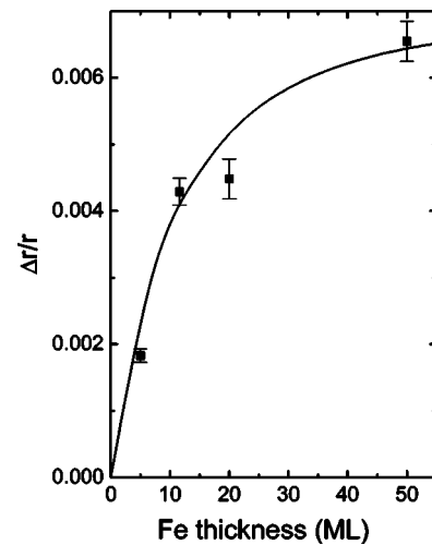
FIG. 7. Fe thickness dependence of the transverse magneto-optical response for Fe/MgO(001) films. The continuous line is a simulation assuming a perfectly continuous film.
