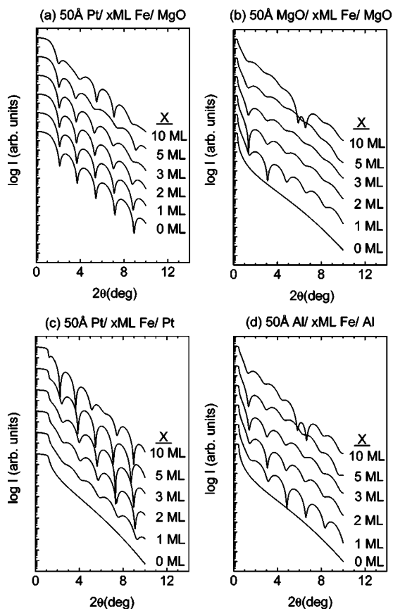
FIG. 1. X-ray reflectivity simulations for a set of ultrathin Fe films of different thickness grown on and capped with different materials. Air-cap, cap-Fe and Fe-substrate interface roughness are 5 Å.
