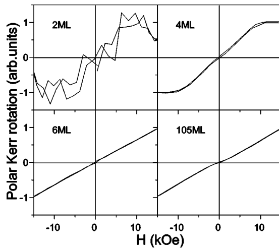
FIG. 5. Polar Kerr hysteresis loops for the 2 ML, 4 ML, 6 ML, and 8 ML samples.
