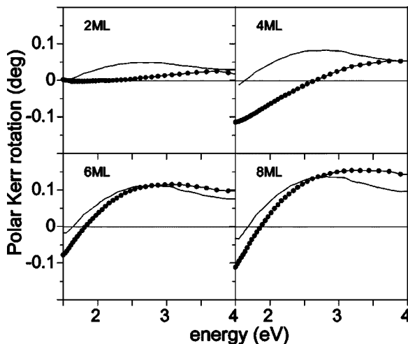
FIG. 6. Polar Kerr spectra for the same samples as Fig. 5; dots: experiment, lines: theoretical simulations assuming a Fe continuous layer 2 ML, 4 ML, 6 ML, and 8 ML thick.
