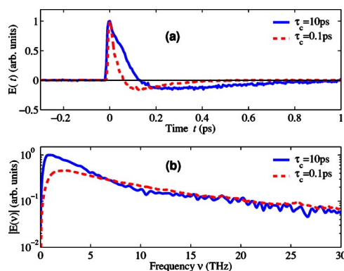
FIG. 6. (Color online) Simulated THz electric field from bulk GaAs at carrier trapping times of \tau_c=10 ps and \tau_c=0.1 ps. In (a) the unfiltered simulated \tau_c=0.1 ps pulse (dashed line) has shorter duration than the 10 ps (solid line). Their Fourier transforms are shown in (b).
