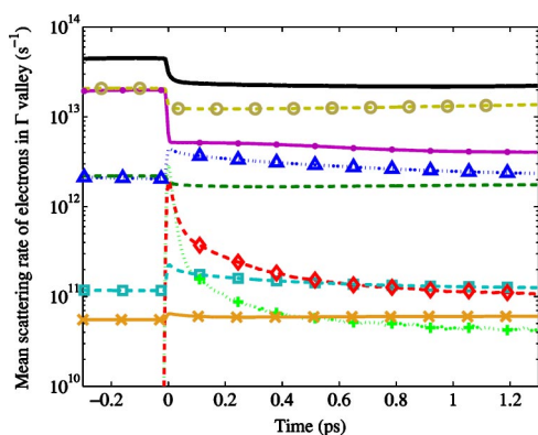
FIG. 4. (Color online) Momentum scattering rates for electrons in the \Gamma valley, with donor and vacancy concentrations of 1 \times 10^{15} \text{ cm}^{-3} each. The rate for each scattering mechanism is averaged over all particles in the simulation, and is plotted as a function of time after laser excitation. The largest contributions to the total rate (solid line) come from electron-hole scattering (circles) and charged impurity scattering (dots). LO-phonon emission (triangles) and absorption (dashed line) are also significant. Acoustic phonon scattering (squares) and vacancy scattering (diagonal crosses) produce lower rates. Least important are TO-phonon absorption (diamonds) and emission (vertical crosses), where in both cases the electronic final state is in the L valley. The infrared pulse arrives at t=0 ps, and produces a step in most scattering rates.
