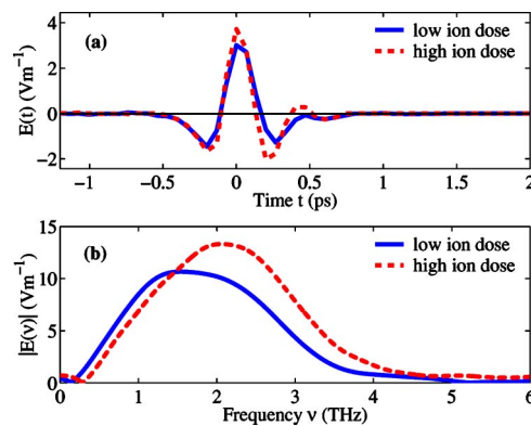
FIG. 2. (Color online) Measured THz electric field E_{\text{THz}} emitted via the surface field mechanism from GaAs: \text{As}^+ samples implanted with low doses (solid lines, 1 \times 10^{13} \text{ cm}^{-2} at 2.4 MeV and 2.5 \times 10^{12} \text{ cm}^{-2} at 1 MeV) and high doses (dotted lines, 5 \times 10^{15} \text{ cm}^{-2} at 2.4 MeV and 1.25 \times 10^{15} \text{ cm}^{-2} at 1 MeV). The time and frequency domain THz electric fields are shown in (a) and (b). The peak electric fields and trailing negative peaks are +3.0 , -1.5 \text{ V m}^{-1} and +3.7 , -2.0 \text{ V m}^{-1} for the low and high dose samples, respectively.
