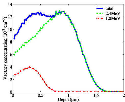
FIG. 1. (Color online) Depth dependence of vacancies (including recoil vacancies) calculated using SRIM software (Ref. 17) for the sample with highest ion dose. The 1 MeV, 2.5 \times 10^{15} \text{ cm}^{-2} dose (dash-dotted line) and 2.4 MeV, 1.0 \times 10^{16} \text{ cm}^{-2} dose (dashed line) create an approximately uniform damage profile (solid line) extending over 1 \mu\text{m} from the surface. By scaling the concentration according to the dose, the distributions for lower dose samples can be obtained.
