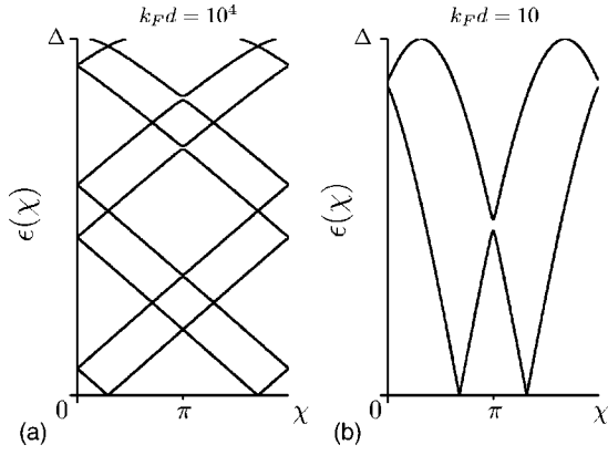
FIG. 1. Spectrum of a clean SFS junction in the perturbative limit \eta=0.1 and for \Delta/E_F=10^{-3} . Two examples are shown: (a) long junction with k_F d=10^4 ( d=5\xi_0 ) and (b) short junction with k_F d=10 ( d=0.05\xi_0 ). Gaps open for \chi=0 and \chi=\pi due to the presence of ordinary reflection. There are two zero energy Andreev levels located at the phase differences \pi \pm \Delta k_{\epsilon=0, \eta} d .
