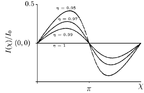
FIG. 6. Current-phase relationships for k_F d = 10 and various spin polarizations in the regime \eta^* < \eta < 1 .
