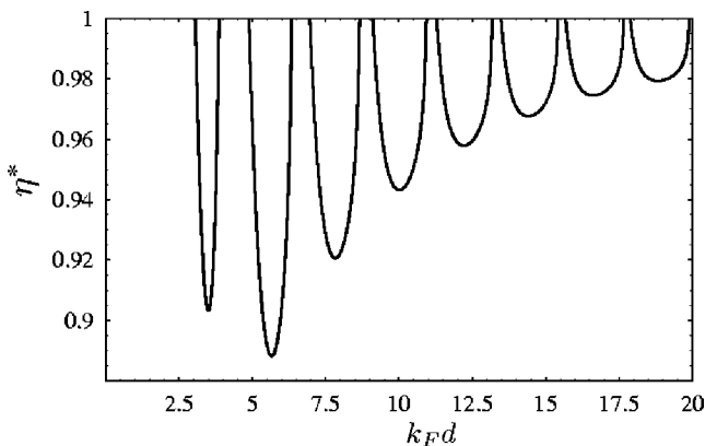
FIG. 4. The zero-energy Andreev states disappear above a critical polarization \eta^* which depends on k_F d . In Sec. III, we show that the current is very close to the quasiclassical estimate with discontinuities when the Andreev level crosses the Fermi level [Fig. 5(a)] for \eta < \eta^* . For \eta > \eta^* , the Josephson current is strongly modified and has no discontinuity, since a gap opens at the Fermi level [Figs. 5(b) and 6]. The minima of \eta^* correspond to values of k_F d \approx (n + 1/2)\pi/\sqrt{2} .
