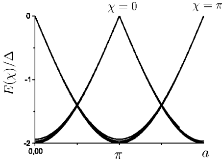
FIG. 7. Zero-state energy E(\chi=0, a) and \pi -state energy E(\chi=\pi, a) for \eta=0.1, 0.3, 0.5 . The intersections of the different curves remain in the vicinity of a=\pi/2 and a=3\pi/2 .
