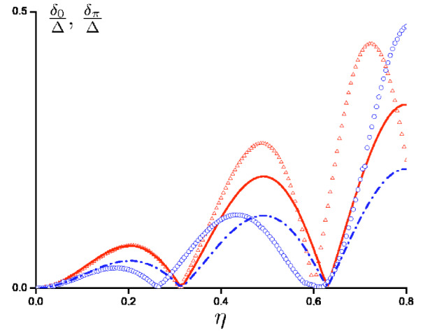
FIG. 2. Gaps at \chi=0 (circles) and \chi=\pi (triangles) as a function of the spin polarization \eta in a short junction with k_F d=10 . Equations (13) and (14) provide a good approximation for small \eta < 0.1 (dash-dotted line, \delta_0 ; solid line, \delta_\pi ).
