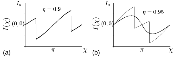
FIG. 5. Zero-temperature current of a short SFS junction with k_F d = 10 . (a) Even for a nearly complete spin polarization \eta = 0.9 , the exact current (thick line) and the quasiclassical approximation (thin line) are identical. (b) For \eta = 0.95 , they are completely different. The natural scale for the current is I_0 = 2e\Delta/\hbar .
