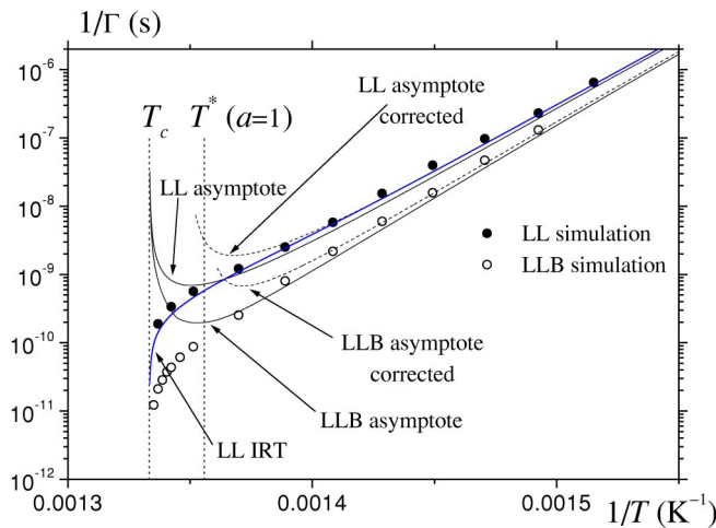
FIG. 1. Switching times for a FePt particle with 8-nm diameter calculated numerically from the LL-Langevin and LLB-Langevin equations and analytically from the appropriate Fokker-Planck equations. While the integral relaxation time (IRT) works very well at all temperatures, the high-barrier asymptotes break down for \sigma \lesssim 1 . The 1/\sigma corrections improve the asymptotes for \sigma \gtrsim 1 .
