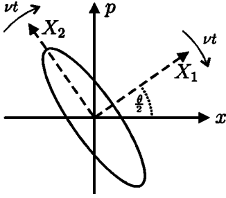
FIG. 1. Representation of the squeezed state |\epsilon=re^{i\theta}\rangle in phase space spanned by the dimensionless position and momentum coordinates. The error ellipse indicates the reduced/enhanced fluctuations for the quadrature components X_1/X_2 .
