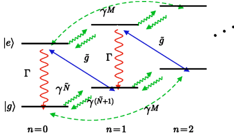
FIG. 4. Coherent and incoherent processes in the squeezed frame as described by master equation (18). In this picture the qubit is only excited on the red sideband ( \tilde{g} ). Followed by a spontaneous decay ( \Gamma ) these transitions cool the resonator to its ground state. The cooling is compensated by the squeezed heat bath which apart from the enhanced heating rate ( \gamma\tilde{N} ) also induces coherences between the states |n\rangle and |n\pm 2\rangle ( \gamma M ).
