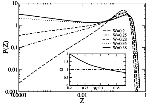
FIG. 7. Distribution of local Kondo temperatures for several levels of disorder. The total number of electrons per unit cell is fixed to 1. The disorder ranges from W=0.2 to 0.38 . We used V=0.5 and E_f=-1.3 , where E_f is measured with respect to the middle of the conduction band. The inset shows the exponent \alpha as a function of the disorder strength. The NFL phase occurs for \alpha \leq 1 .
