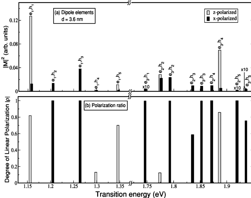
FIG. 2. (a) Matrix elements squared and (b) degree of linear polarization for the interband transitions h_i \rightarrow e_j ( i=1, \dots, 5, j=1, 2, 3 ), as a function of the transition energy for the d=3.6 nm InAs wire.
