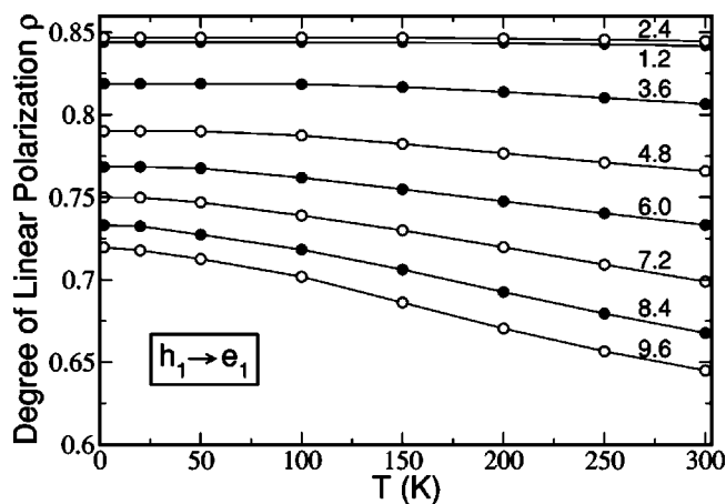
FIG. 5. Degree of linear polarization of the fundamental transition h_1 \rightarrow e_1 as a function of temperature T for the different wire diameters considered.
