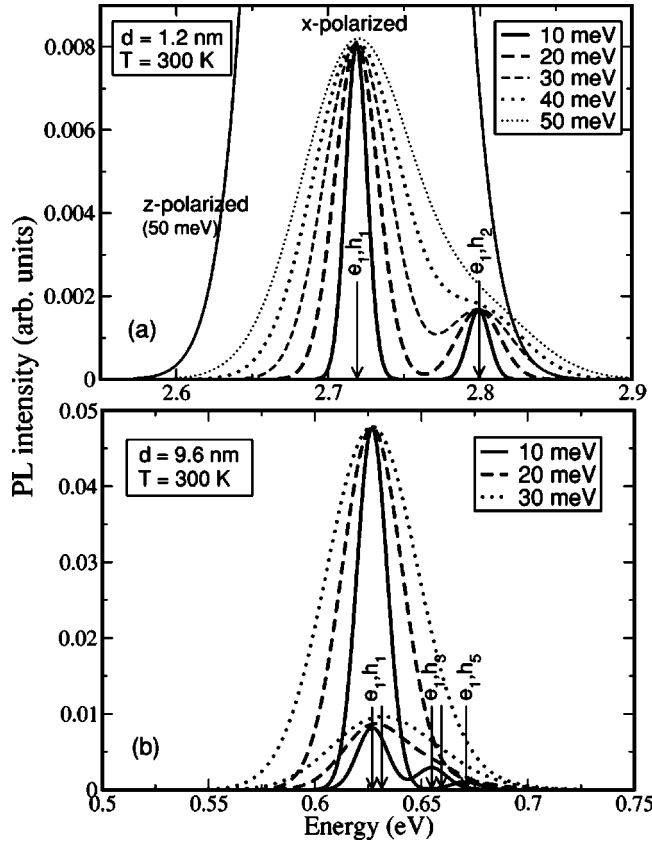
FIG. 7. PL polarization spectra at T=300 K calculated for a d=1.2 nm (a), and a d=9.6 nm (b) wire for different values of the line broadening.
