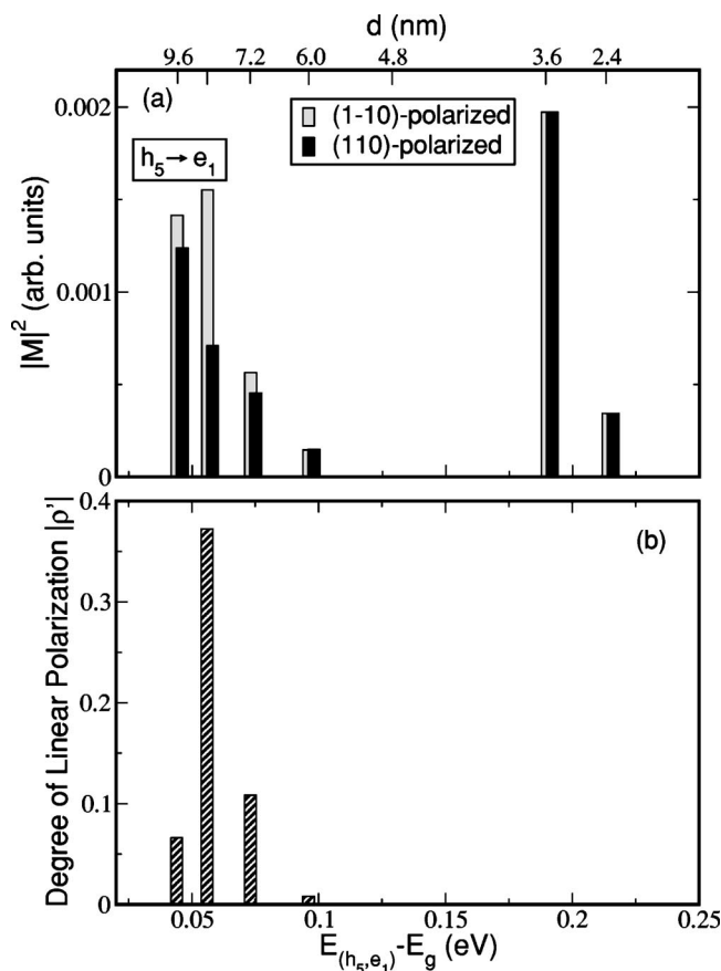
FIG. 9. (a) In-plane matrix elements squared and (b) degree of linear polarization for the interband transitions h_5 \rightarrow e_1 , as a function of the transition energy measured from the band gap (lower x axis) and wire diameter (upper x axis), in D_{2d} InAs wires.
