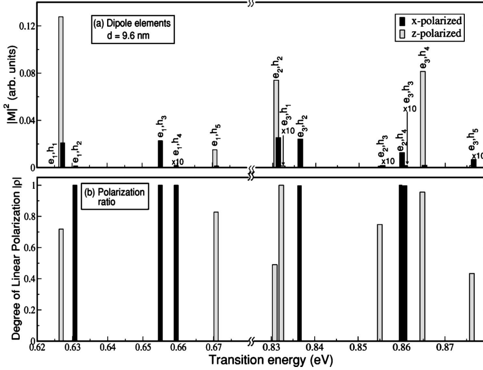
FIG. 3. (a) Matrix elements squared and (b) degree of linear polarization for the interband transitions h_i \rightarrow e_j ( i=1, \dots, 5 , j=1, 2, 3 ), as a function of the transition energy for the d=9.6 nm InAs wire.
