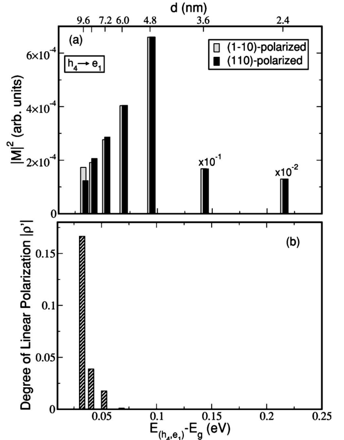
FIG. 8. (a) In-plane matrix elements squared and (b) degree of linear polarization for the interband transitions h_4 \rightarrow e_1 , as a function of the transition energy measured from the band gap (lower x axis) and wire diameter (upper x axis), in D_{2d} InAs wires.
