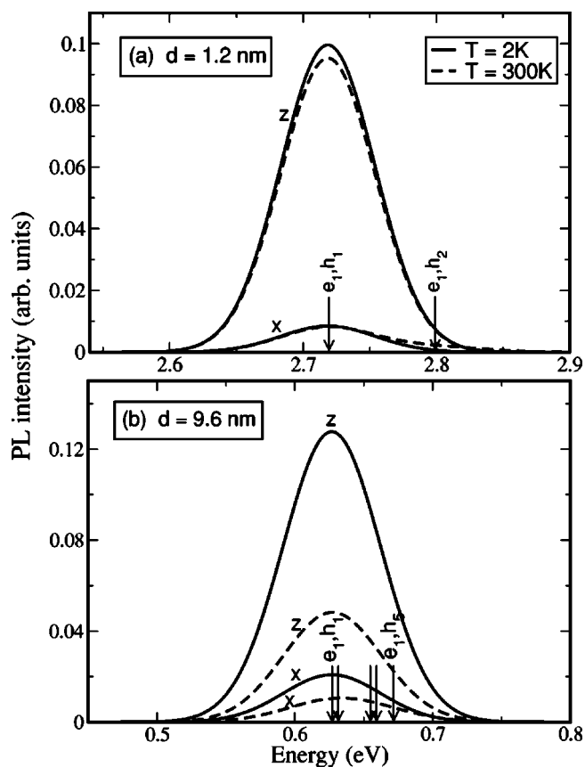
FIG. 6. PL polarization spectra around the energy of the fundamental h_1 \rightarrow e_1 transition, calculated at T=2 K and T=300 K for a (a) d=1.2 nm and a (b) d=9.6 nm wire (with 50 meV broadening). The arrows mark the position in energy of the transitions h_i \rightarrow e_1 with i=1, \dots, 5 .
