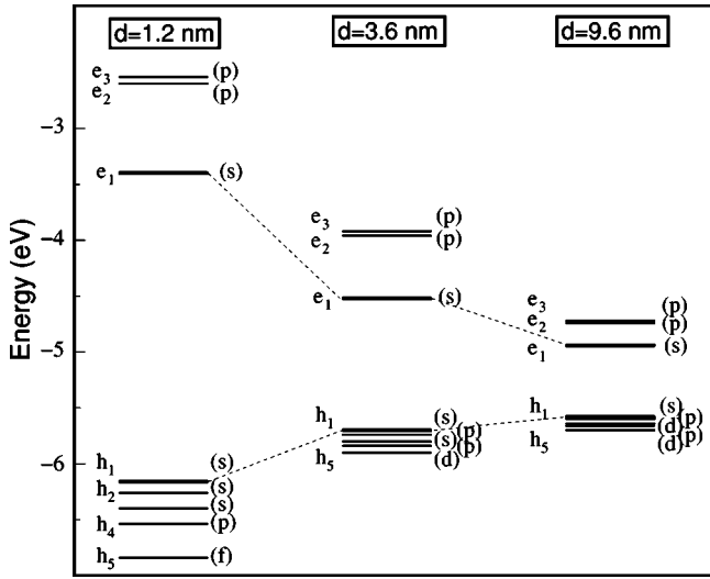
FIG. 1. Schematics of the calculated single-particle energy levels (labeled with their main angular momentum component) for 3 InAs D_{2d} cylindrical wires with sizes d=1.2, 3.6, 9.6 nm, respectively. The dashed lines connect, respectively, CBM and VBM in the different wires. Only a few states are shown that were used in the calculations of the optical properties.
