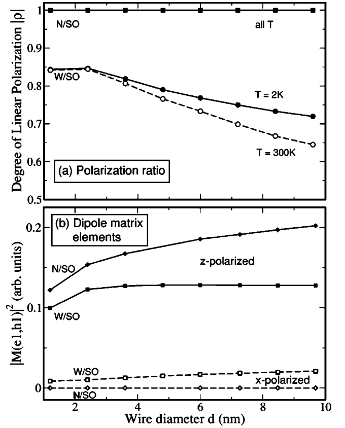
FIG. 4. (a) Degree of linear polarization of the fundamental transition h_1 \rightarrow e_1 as a function of wire diameter, calculated at T=2 K and T=300 K both considering (W/SO) and not considering (N/SO) SO splitting. (b) Dipole matrix elements, for the same transition, polarized parallel ( z ) and perpendicular ( x ) to the wire axis, in the finite and zero SO splitting approximations.
