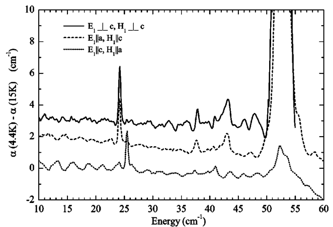
FIG. 2. Differential absorption in \mathbf{E}_1 \perp \mathbf{c} (two upper curves) and \mathbf{E}_1 \parallel \mathbf{c} (lower curve) polarization. Spectra have been offset in the vertical direction.
