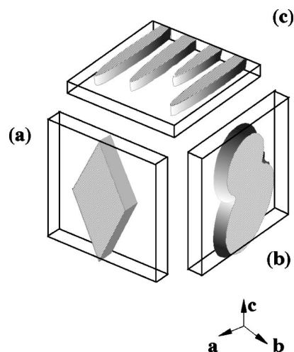
FIG. 8. Different shape of domain boundaries in thin films viewed from three principle axes. (a) The observation direction is the [100] zone axis. The domain boundary takes a zigzag pattern, or diamond-shape elongated to the c -axis direction. (b) The [010] zone axis direction, rounded shape, and (c) the [001] zone-axis direction, the lamella or layer structure.
