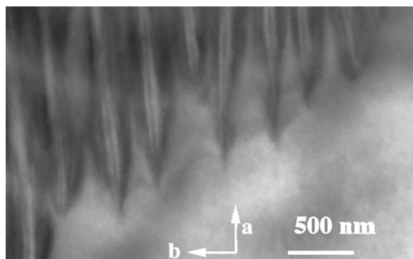
FIG. 4. The phase separated state observed at 110 K at the [001] zone axis direction of the specimen for x=0.39 . The crystallographic a -axis direction and b -axis direction are indicated. The lower part is the monoclinic phase. The crystallographic type of lamella domains is uncertain, since the patterns in the CBED are distorted.
