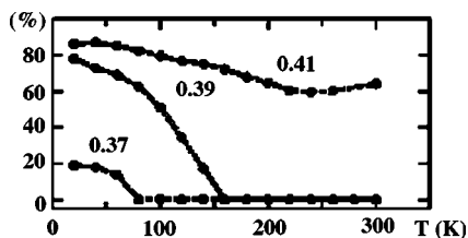
FIG. 1. Volume fraction of the low temperature orthorhombic (LTO) phase in the specimens for x=0.37 , 0.39 , and 0.41 of Y_{1-x}Ca_xTiO_3 obtained from the x-ray powder diffraction experiments. The LTO phase appears below the insulator-to-metal transition temperatures ( T_{MI} ), and the two-phase state with the monoclinic phase takes place. On further cooling the volume fraction of the LTO phase increases (Ref. 16).
