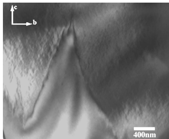
FIG. 6. Electron microscope image at the [100] zone axis direction taken at 110 K of the specimen for x=0.39 . The domain with high strain and wavy contrast is visible at the upper part. The lower domain without strain and wavy contrast was identified as a monoclinic phase by CBED pattern.
