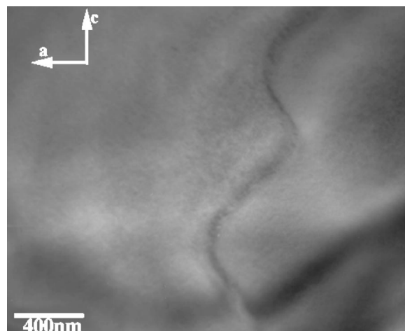
FIG. 5. Two kinds of domains observed at 110 K at the [010] zone axis direction of the specimen for x=0.39 . The crystallographic a -axis direction and c -axis direction are indicated. The wavy domain boundary is seen at the center. The left-hand side is the strained domain, and the right-hand side is the monoclinic phase.
