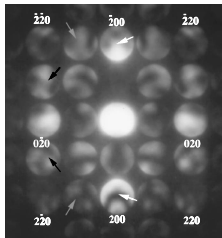
FIG. 3. CBED pattern taken at 150 K at the [001] zone axis direction of the specimen for x=0.39 . Horizontal asymmetry in the pattern is observed, whereas the vertical mirror symmetry in the pattern is conserved. Arrows indicate example positions, where the absences in horizontal mirror symmetry in contrast are observed. This change in CBED pattern is due to the transition to a monoclinic lattice.
