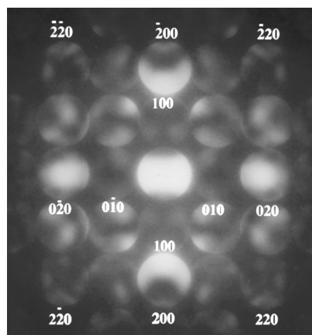
FIG. 2. CBED pattern taken at room temperature at the [001] zone axis of the specimen with x=0.39 . Both horizontal and vertical mirror symmetries in the CBED pattern are observed.
