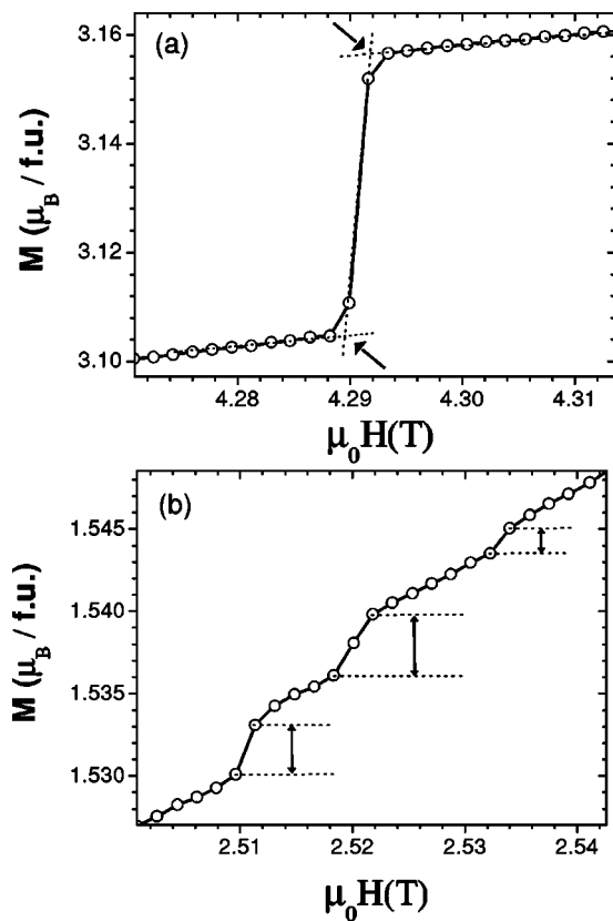
FIG. 3. Illustration of the constructions used to evaluate the height of the magnetization jumps. For large steps (a), \Delta M is derived from the intersection points denoted by the arrows (see text). For small steps (b), \Delta M is directly estimated from the data points flanking the jumps, as denoted by the arrows.
