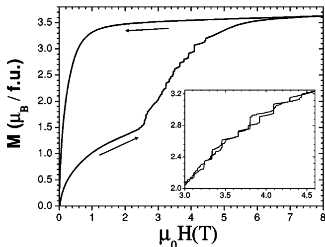
FIG. 1. M(H) loop recorded at T=1.5 K, after a zero-field cooling, on \text{Pr}_{0.6}\text{Ca}_{0.4}\text{Mn}_{0.96}\text{Ga}_{0.04}\text{O}_3 . The arrows indicate the directions of the field variation. The inset is an enlargement of the field-increasing branches of two independent runs recorded on the same sample.
