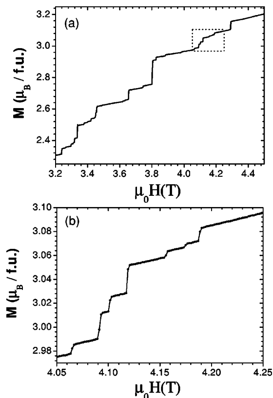
FIG. 2. Field-increasing branch of a M(H) loop at T=1.5 K, shown at two scales: (b) is an enlargement of the dotted window drawn in (a).
