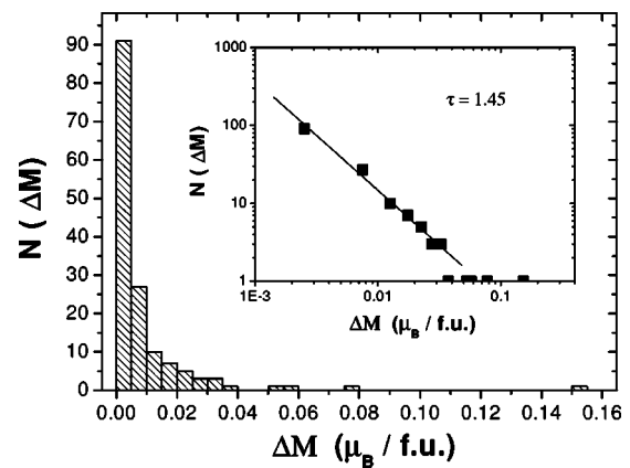
FIG. 4. Histogram of the distribution of magnetization jumps along the field-increasing branch of an M(H) loop at 1.5 K (main panel). The inset shows the same data in a log-log plot. The solid line is a fit corresponding to a power law N(\Delta M) \propto \Delta M^{-\tau} , with \tau = 1.45 .
