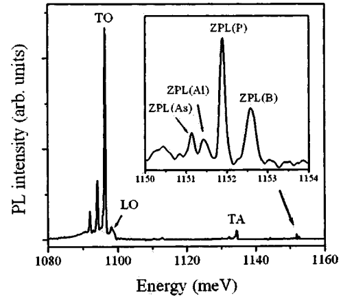
FIG. 1. Photoluminescence from Czochralski-grown isotopically enriched ^{30}\text{Si} . The ZPL region is expanded in the inset. TA, LO, and TO label the wave-vector conserving phonon sidebands which are predominantly created by the boron. The spectra are not corrected for the spectrometer response.
