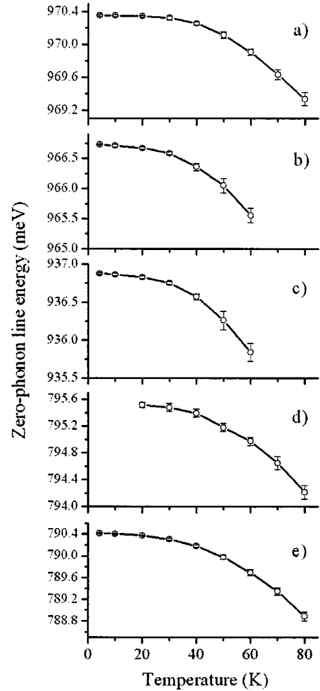
FIG. 4. Temperature dependence of (a) the “G” line, (b) the “I” line (c) the “T” line, (d) the “C” line (from an excited state of the “C” center), and (e) the “C” line. All data are measured using ^{30}\text{Si} .
