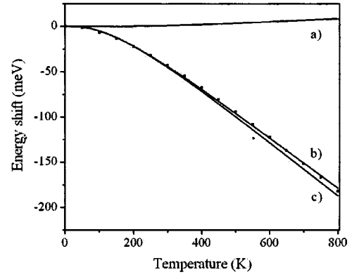
FIG. 2. Points show representative data for the temperature dependence of the indirect energy gap (Ref. 9). Line (a) is the contribution from the shift caused by lattice expansion. Line (c) is the shift term \Delta E_g^{\text{EP}} , calculated from Eq. (7), and scaled so that the total shift [line (b)] has a best fit to the datum points.
