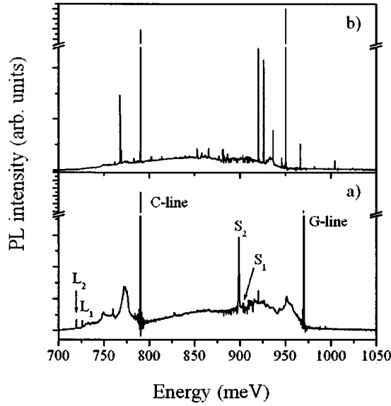
FIG. 3. Photoluminescence from electron-irradiated ^{30}\text{Si} (a) before and (b) after annealing at 400^\circ\text{C} for 30 min. L_1 and L_2 are the LVMs of the C-line with quanta 64.0 and 70.6 meV; S_1 and S_2 are the LVMs of the G-line with quanta 66.4 and 71.3 meV, respectively. The sharp absorption lines at about 900 meV are due to atmospheric absorption. The spectra are not corrected for the spectrometer response.
