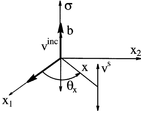
FIG. 3. Scalar problem of the shear wave interacting with a screw dislocation.
