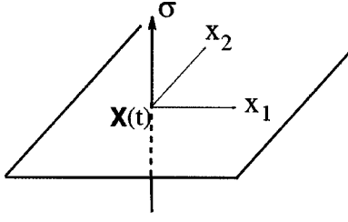
FIG. 2. Configuration of the 2D problem.
