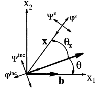
FIG. 6. Acoustic wave ( v_\alpha velocity) and in-plane shear-wave ( v_\beta velocity) interacting with a distribution of gliding edge dislocations. The n th dislocation is characterized by its mean position X_0^n and its in plane Burgers vector b^n .
