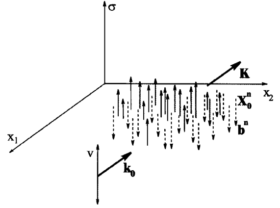
FIG. 4. Scalar problem of the shear wave interacting with a distribution of screw dislocations (solid arrows correspond to positive Burgers vectors and dotted arrows correspond to negative Burgers vectors).
