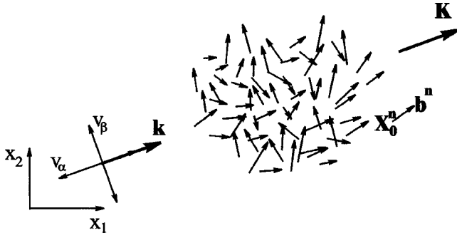
FIG. 5. Acoustic wave ( v_\alpha velocity) and in-plane shear-wave ( v_\beta velocity) interacting with a 2D gliding edge dislocation.
