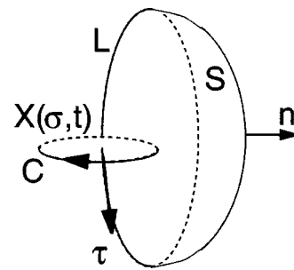
FIG. 1. Definition of the Burgers vector.
