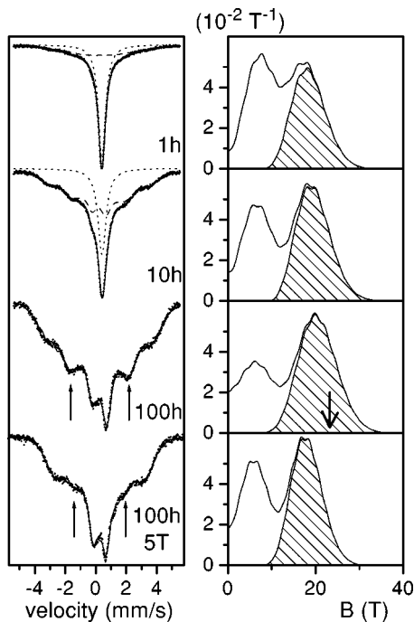
FIG. 1. 4.2 K Mössbauer spectra of FeAl ball-milled for different times. Full, broken, and dotted lines are fitted curves of the full spectra and the magnetic and the paramagnetic components, respectively. In the hyperfine field distributions fitted to the magnetic components shading and an arrow marks the hyperfine field of Fe atoms with localized moments and that of Fe atoms with 4 Al–4 Fe nearest neighbors in \text{Fe}_3\text{Al} (Ref. 19), respectively. The positions of the second and fifth lines for the high field peak in the spectra of the 100 h sample in 0 T and 5 T field are marked as well.
