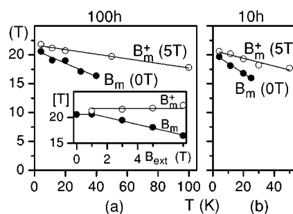
FIG. 5. Temperature dependence of the hf of the localized Fe magnetic moments in 0 T ( B_m , dots) and in 5 T ( B_m^+ , circles) for the 100 h (a) and 10 h (b) ball-milled FeAl, respectively. The inset shows the external field dependence of B_m (dots) at 4.2 K; it is corrected for the applied field and the canting angle as explained in the text ( B_m^+ , circles).
