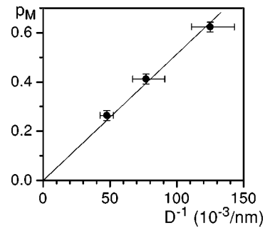
FIG. 2. The fraction of magnetic Fe atoms, p_M , in the ball-milled FeAl alloys as a function of the inverse grain size, D^{-1} . The proportionality is shown by the full line.
