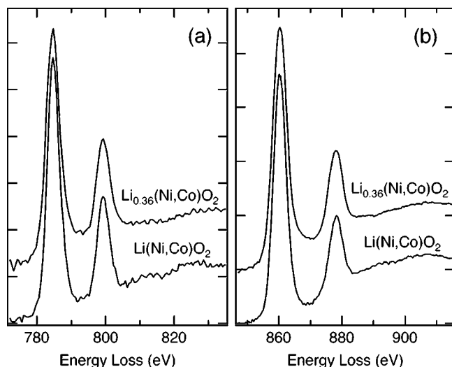
FIG. 6. (a) Co and (b) Ni white lines in stoichiometric \text{LiNi}_{0.8}\text{Co}_{0.2}\text{O}_2 and delithiated \text{Li}_{0.36}\text{Ni}_{0.8}\text{Co}_{0.2}\text{O}_2 .
