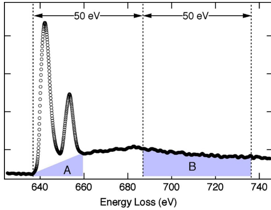
FIG. 1. (Color online) Mn L_{2,3} edge from MnO_x showing the free-electron-like contributions to the white-line intensity (region A) and a 50 eV window located 50 eV above the L_3 onset (region B), which was used to normalize the white-line intensity.
