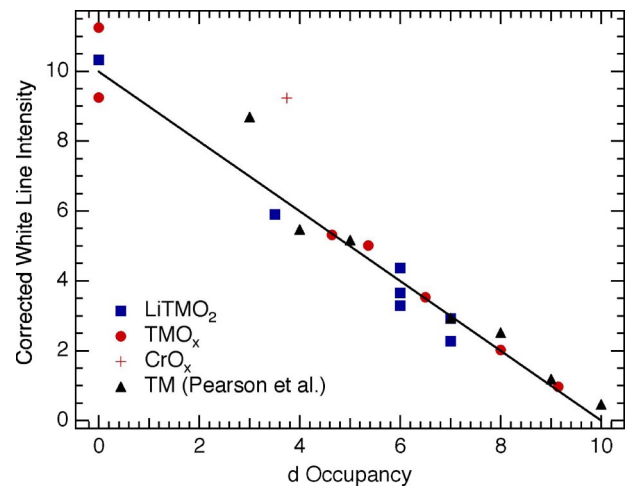
FIG. 5. (Color online) Normalized white-line intensity for a series of transition metals, transition-metal oxides, and lithium transition-metal oxides plotted vs d occupancy. The solid line represents the expected white-line line intensity based upon Eq. (4).
