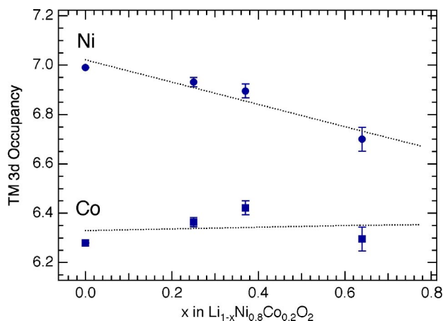
FIG. 7. (Color online) Nickel and cobalt 3d occupancies in \text{Li}_{1-x}\text{Ni}_{0.8}\text{Co}_{0.2}\text{O}_2 .
