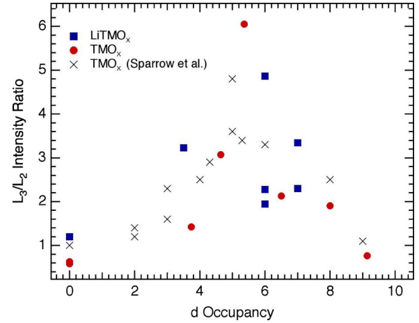
FIG. 4. (Color online) White-line ratio for a series of transition-metal oxides and lithium transition-metal oxides. The data of Sparrow et al. are from (Ref. 28).
