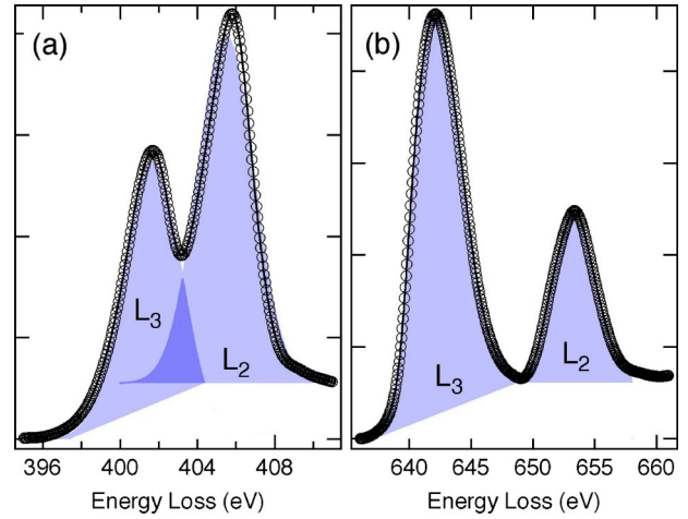
FIG. 2. (Color online) (a) Sc L_{2,3} edge from ScO_x showing the typical Gaussian fit and integration windows (shaded) used to determine the L_3/L_2 ratio in the early transition metals and Cu. (b) Mn L_{2,3} edge from MnO_x showing the typical integration windows (shaded) used to determine the L_3/L_2 ratio in the middle transition metals.
