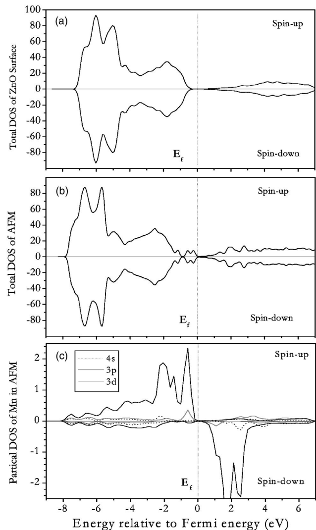
FIG. 2. Total DOS for (a) pure and (b) Mn-doped ZnO thin film in the antiferromagnetic ground state. The corresponding partial DOS of Mn atom is shown in (c).
