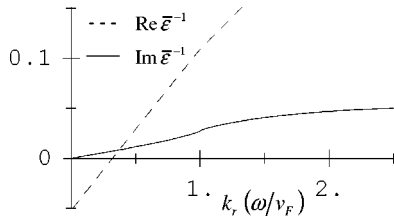
FIG. 1. Inverse surface dielectric function \bar{\varepsilon}(\omega, k_r)^{-1} (the real and imaginary parts) plotted against parallel wave vector k_r for \hbar\omega = 2 eV.
