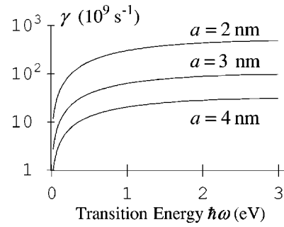
FIG. 2. Relaxation rate \gamma of QD at a distance a from metal surface as a function of transition energy \hbar\omega . The distances a to the surface are indicated at the corresponding curves. The computations are made for a constant d_{12} = 28 \times 10^{-18} esu, which corresponds \gamma_0 = 10^9 s ^{-1} at \hbar\omega = 2 eV.
