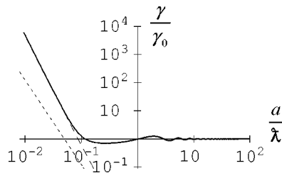
FIG. 3. Relaxation rate \gamma of QD at a distance a from metal surface relative to \gamma_0 for isolated QD computed from Eqs. (15) and (17) by numerical integration for \hbar\omega = 2 eV (bold line). The long-dash line is the asymptotic given by the second term and short-dash line by the first term in the brackets of Eq. (16). Note the double logarithmic scale.
