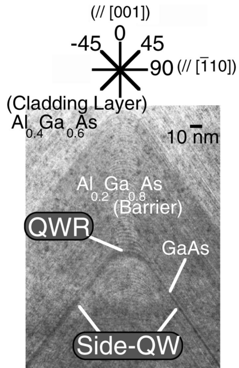
FIG. 1. Cross-sectional transmission electron microscope (TEM) image of a ridge quantum wire (QWR) laser. QWR is formed at the ridge corner of two adjacent QWs (side-QWs). We define \theta = 0^\circ as the growth ([001]) direction and \theta = \pm 90^\circ as the [1\bar{1}0] direction.
