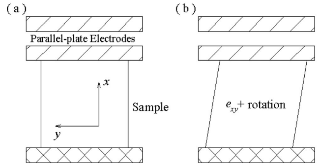
FIG. 3. (a) Schematic illustration of the experimental setup for the capacitance measurement. In this configuration, we can measure the change in the length along the x direction. (b) Experimental setup for measuring e_{xy} across T_Q .
