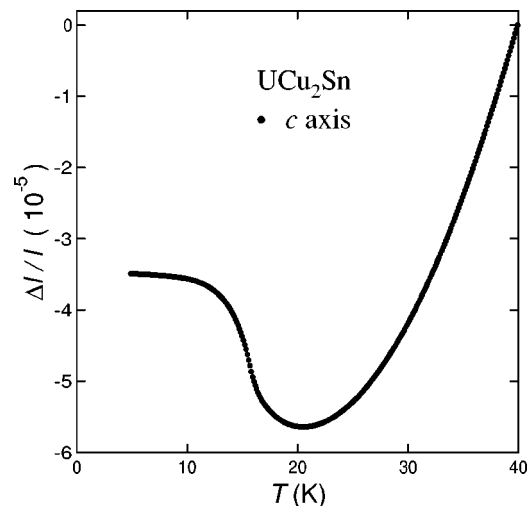
FIG. 4. Temperature dependence of thermal expansion \Delta l/l along the c axis.
