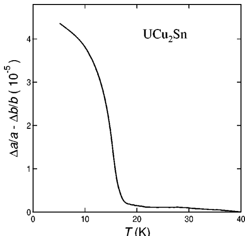
FIG. 2. Temperature dependence of \Delta a/a - \Delta b/b .
