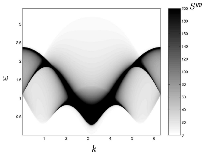
FIG. 9. Structure factor S^{yy} as a function of k and \omega for anisotropy \Delta=0.25 and external magnetic field H=0.8J .
