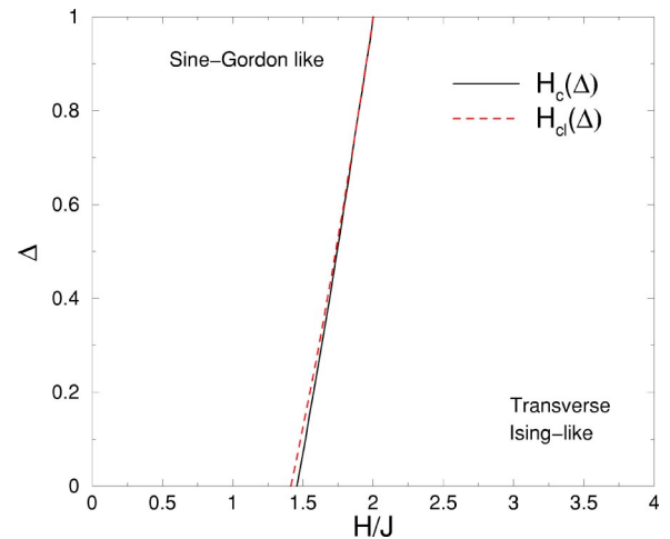
FIG. 2. Mean-field phase diagram. The critical line is denoted by H_c(\Delta) and the classical line by H_{cl}(\Delta) .
