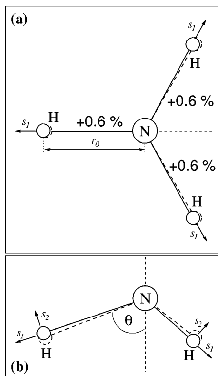
FIG. 2. Calculated structure of NH 3 (solid lines) compared with the experimental structure (dashed lines), (a) Top view, (b) side view, cutting through one of the N-H bonds. N-H distances ( r_0 ) are given as percentage deviations from the experimental value (1.012 Å). The calculated value of \theta is 68.2°, the experimental value is 67.9°. s_1 and s_2 are the two degrees of freedom employed in the calculation of the dynamical matrix as discussed in the text.
