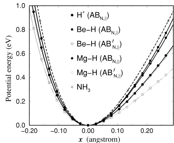
FIG. 8. Calculated potential energy curves for N-H bond-stretching modes for AB_{N\parallel} and AB'_{N\parallel} configurations. Solid symbols are calculated points for H at the AB_{N\parallel} site and the thick solid lines are the corresponding fourth-order polynomial fits [Eq. (4)]. Open symbols and thin solid lines are the calculated points and fits for H at the AB'_{N\parallel} site. The potential energies are set to zero at the equilibrium position of each structure. The star symbols and dashed line indicate the potential energy curve for the NH_3 symmetric stretch mode, included for comparison.
