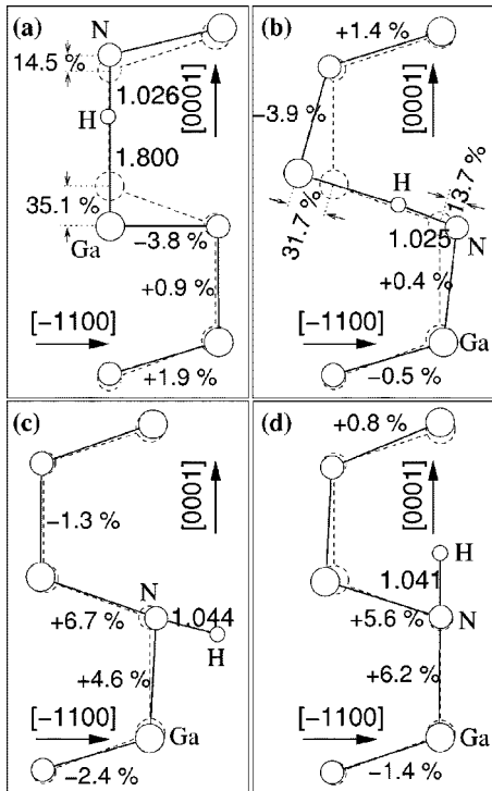
FIG. 4. Schematic representation of atomic positions in the (11-20) plane for H^+ at (a) BC_{\parallel} site, (b) BC_{\perp} site, (c) AB_{N_{\perp}} site, and (d) AB_{N_{\parallel}} site in wurtzite GaN. The configurations are depicted in order of increasing energy (see Table III). Large circles represent Ga atoms, medium circles N atoms, and the small circles H atoms. Dashed circles indicate ideal atomic positions, dashed lines bonds in the ideal lattice. Distances between H and its neighbors are given in Å, changes in Ga-N bond lengths are given as a percentage of change from the bulk Ga-N bond lengths.
