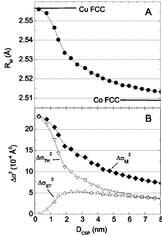
FIG. 7. Results based on the model to estimate the particle size. As the size of the particle increases, the coordination distance (A) and Debye-Waller factor (B) change from values similar to the bulk Cu to values similar to the bulk Co. In panel (B) are displayed the static ( \Delta ) and thermal ( \nabla ) contributions for the total ( \blacklozenge ) Debye-Waller factor.
