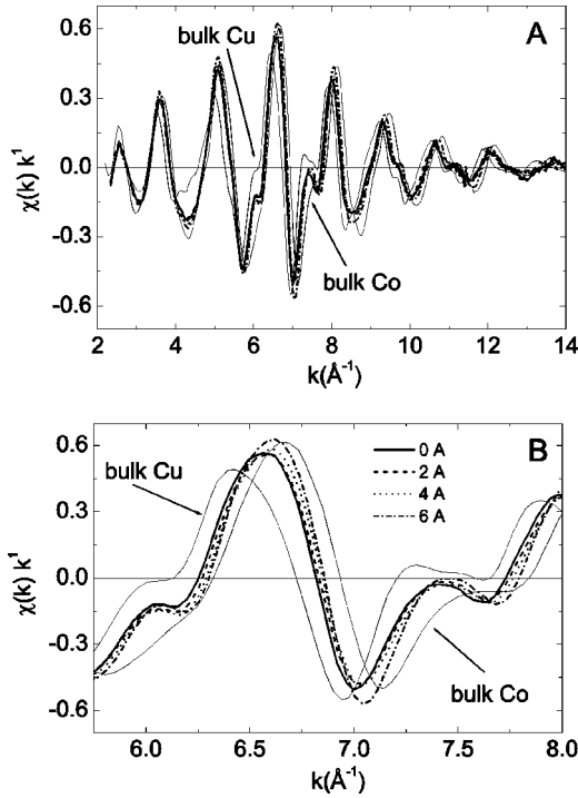
FIG. 4. XAFS signal extracted from the raw absorption spectra of some representative \text{Co}_{10}\text{Cu}_{90} samples. The upper panel displays the signal in the whole range used in the data analysis, while the bottom panel shows an enlarged region, where one can compare the signal of the samples with those of bulk Cu and Co.
