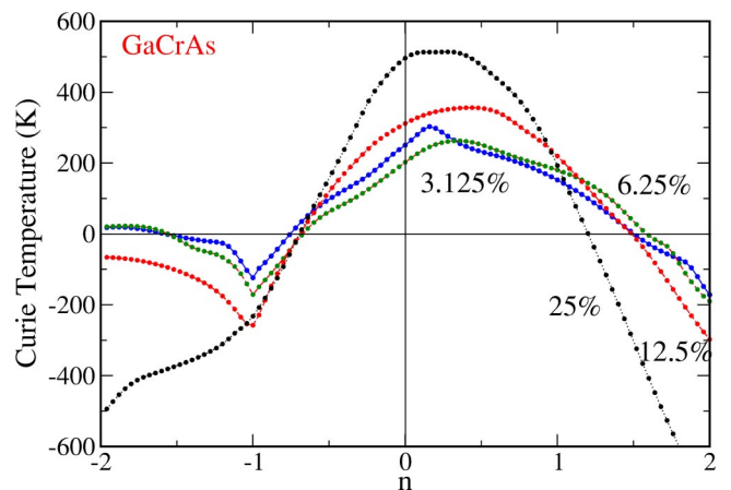
FIG. 10. T_C^{\text{MF}} of (Ga,Cr)As with different Cr concentrations as a function of the electron number n . n=0 corresponds to the system \text{Ga}_{1-x}\text{Cr}_x\text{As} with no additional donor or acceptor defects.
