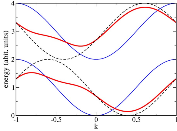
FIG. 1. The energy bands (thick solid line) of the spiral structure with \mathbf{q}=0.4 , \Delta=2 , and \theta=45^\circ . H(\mathbf{k})=1-\cos(\pi\mathbf{k}) . The thin solid lines show the bands of a ferromagnetic configuration. The broken lines give the ferromagnetic bands shifted in the reciprocal space according to the given \mathbf{q} (see the text). The minimal energy of the ferromagnetic configuration is lower than for the spiral. On the other hand, the maximal energy of the ferromagnet is higher than for the spiral.
