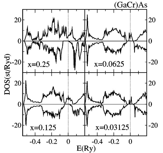
FIG. 4. The DOS of \text{Ga}_{1-x}\text{Cr}_x\text{As} . The DOS is given per unit cell of the zinc blende crystal structure. The DOS above (below) the abscissas axis corresponds to the spin-up (down) states.
