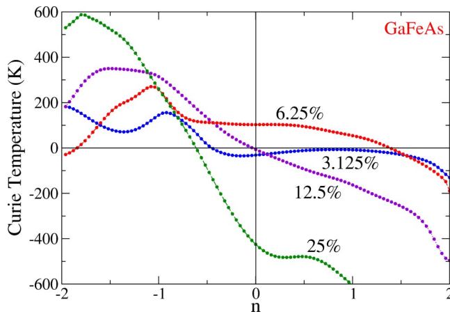
FIG. 13. T_C^{\text{MF}} of (Ga,Fe)As with different Fe concentrations as a function of the electron number n . n=0 corresponds to the system \text{Ga}_{1-x}\text{Fe}_x\text{As} with no additional donor or acceptor defects.
