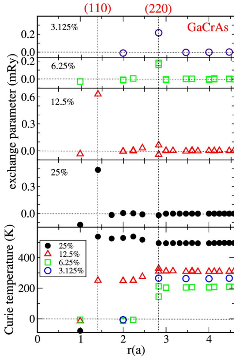
FIG. 6. The parameters of the exchange interaction between Cr atoms (upper panel) and the variation of T_C^{\text{MF}} with increasing number of the contributing coordination spheres (lower panel). The abscissa gives the radius of the coordination sphere in the units of the lattice parameter of the zinc blende crystal structure. The calculations has been performed up to r=7a . Because of very small values the exchange parameters for large r are not shown. The broken vertical lines show the coordination spheres with strongest exchange interaction with the central atom. Two data points for the same system and the same radius (e.g., at r=2.828a for x=12.5\% and) mean that there are two inequivalent coordination spheres with equal radii.
