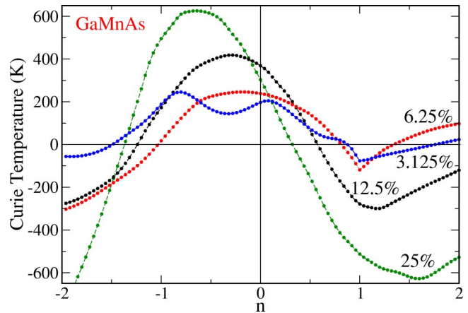
FIG. 2. T_C^{\text{MF}} of (Ga,Mn)As with different Mn concentrations as a function of the electron number n . n=0 corresponds to the system \text{Ga}_{1-x}\text{Mn}_x\text{As} with no additional donor or acceptor defects.
