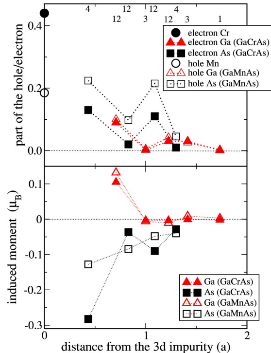
FIG. 5. Distribution of the carrier states over atoms (upper panel) and induced magnetic moments (lower panel) for \text{Ga}_{1-x}\text{Cr}_x\text{As} and \text{Ga}_{1-x}\text{Mn}_x\text{As} with x=3.125\% . For (GaCr)As, the distribution is given for the occupied (electron) states in the impurity band. For (GaMn)As, the distribution is given for empty (hole) states in the valence band. All values are for the coordination spheres. The numbers of atoms in the coordination spheres are shown at the top of the picture. The calculated values for (GaMn)As are taken from I.
