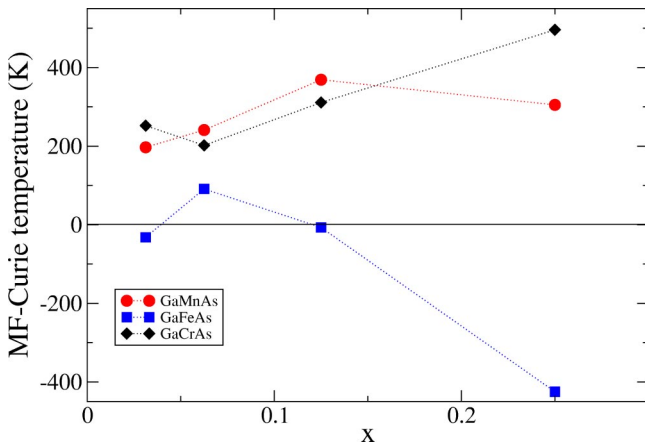
FIG. 8. T_C^{\text{MF}} of (Ga,Cr)As, (Ga,Mn)As, and (Ga,Fe)As for different concentrations of the 3d impurity.
