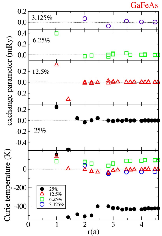
FIG. 12. The parameters of the exchange interaction between Fe atoms (upper panel) and the variation of T_C^{\text{MF}} with increasing number of the contributing coordination spheres (lower panel). The abscissa gives the radius of the coordination sphere in the units of the lattice parameter of the zinc blende crystal structure. The decay of the exchange parameters is illustrated in the logarithmic scale in Fig. 7.
