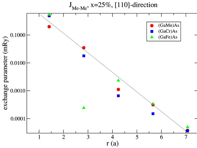
FIG. 7. The absolute values of the exchange parameters between 3d impurities as a function of the interatomic distance. The impurity concentration is 25%. The [110] crystallographic direction is presented. A logarithmic ordinate axis is used to visualize fast decay of the exchange parameters. The small value of the exchange parameter of (GaFe)As at r=2\sqrt{2}a results from the oscillation of the parameter as a function of r (Fig. 12). The dashed straight line is a guide for the eye.
