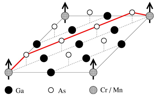
FIG. 9. The z=0 and z=a/4 planes of the supercell for the concentration of magnetic impurity of 3.125%. The exchange path shown by the thick line connecting the impurity atoms goes over As atoms.
