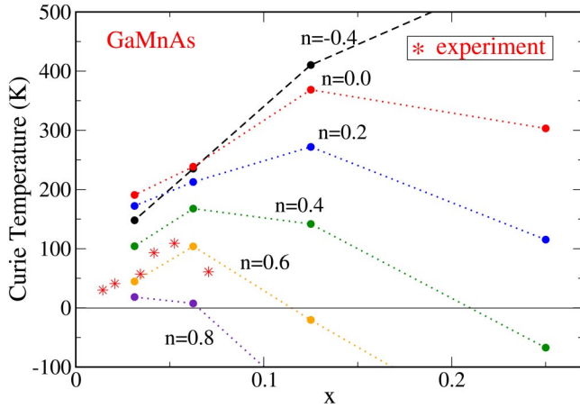
FIG. 3. T_C^{\text{MF}} of (Ga,Mn)As as a function of the Mn concentration x for different electron numbers n . n is defined as in Fig. 2. Note that the number of holes p per Mn atom equals 1 - n . The stars show the experimental values of the Curie temperature.
