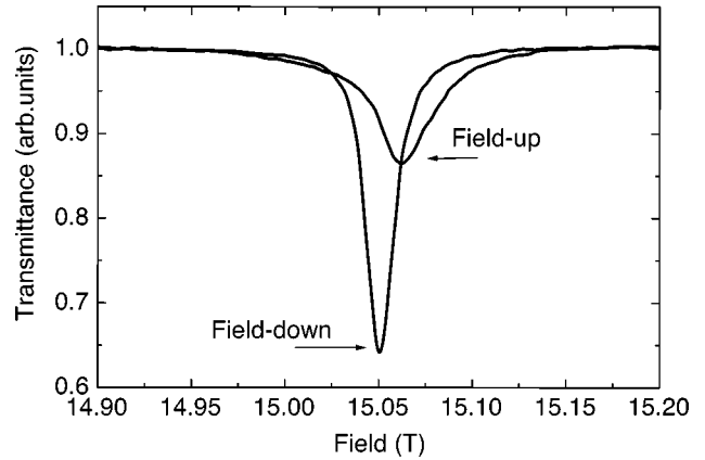
FIG. 1. The ESR spectrum in \text{CuGeO}_3 taken at a frequency of 431.8 GHz in ascending and descending fields ( T=4.2 K). The spectrum clearly indicates a magnetic field hysteresis.
