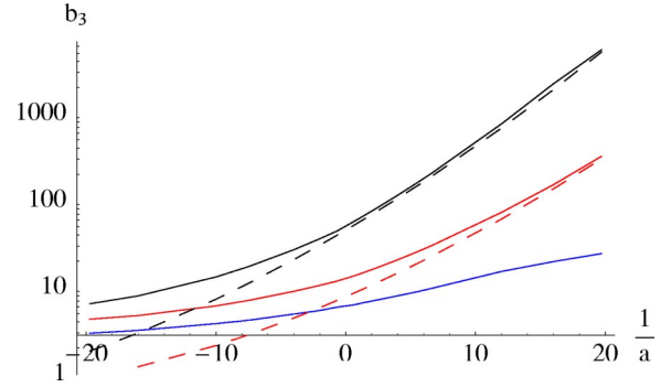
FIG. 4. b_3 as a function of the inverse scattering length 1/a , in units of eV, for three values of H ( \Lambda=200 eV) (solid lines, H = -3.23, -0.22, 0.05 , from bottom to top). The dashed line is the estimate e^{\beta B_3} .
